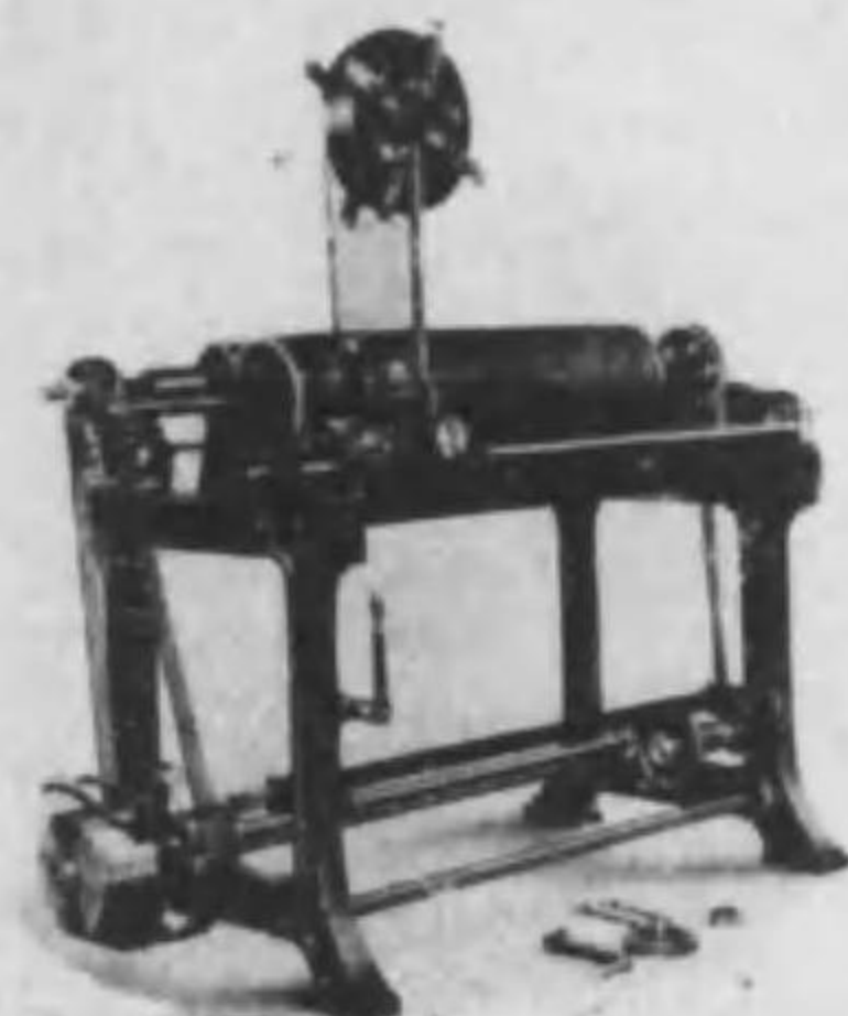
Saw-Tooth-Wire Mounting, Grinding, Dressing and Burnishing Machine.
