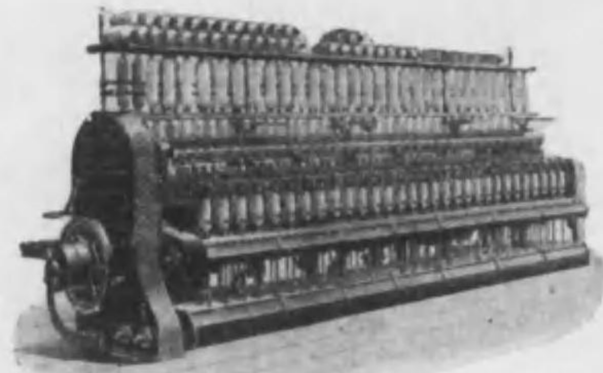
Intermediate Frame
