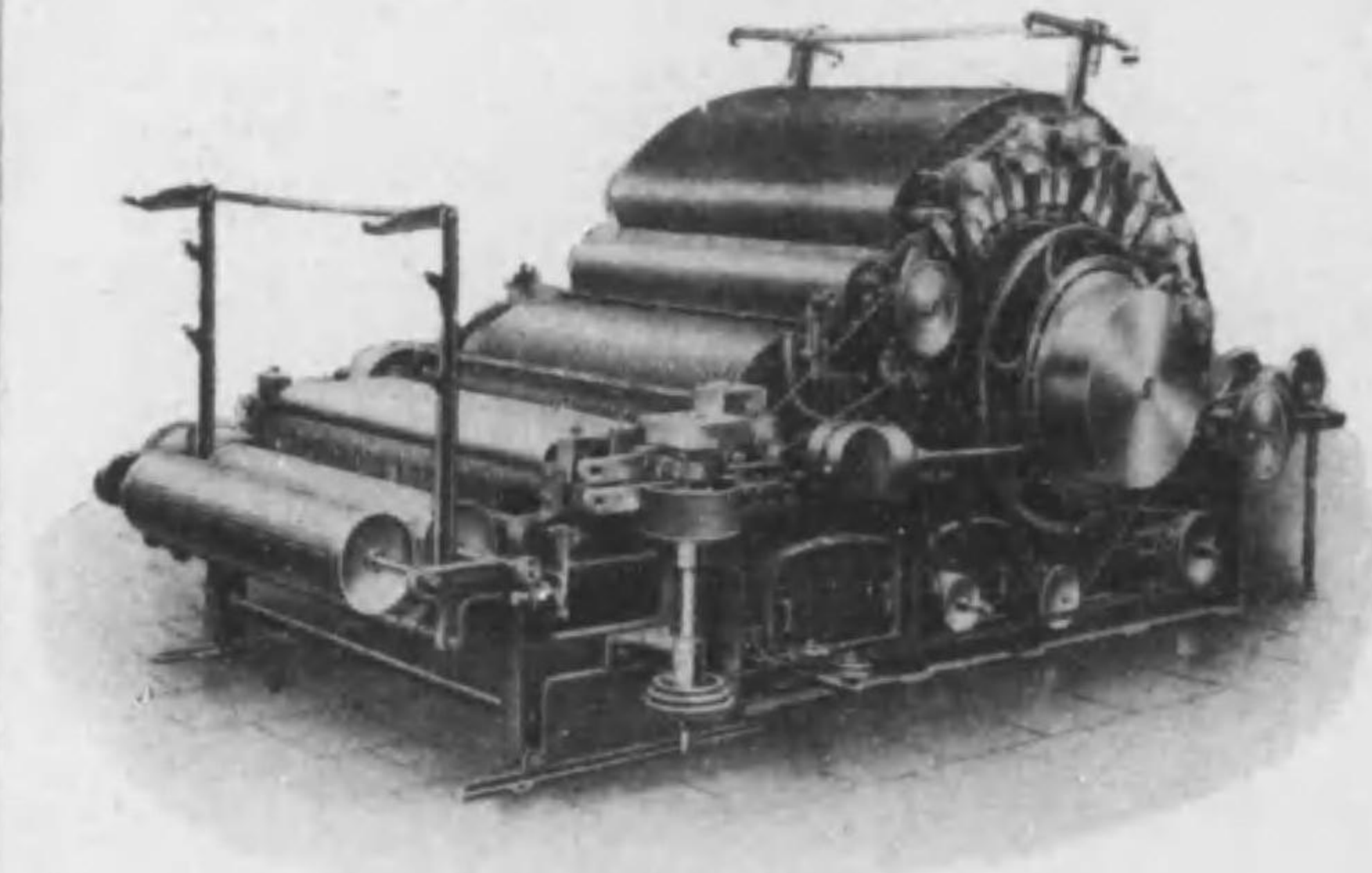
SINGLE-FINISHING CARDING ENGINE fitted with improved ring doffer Condenser
