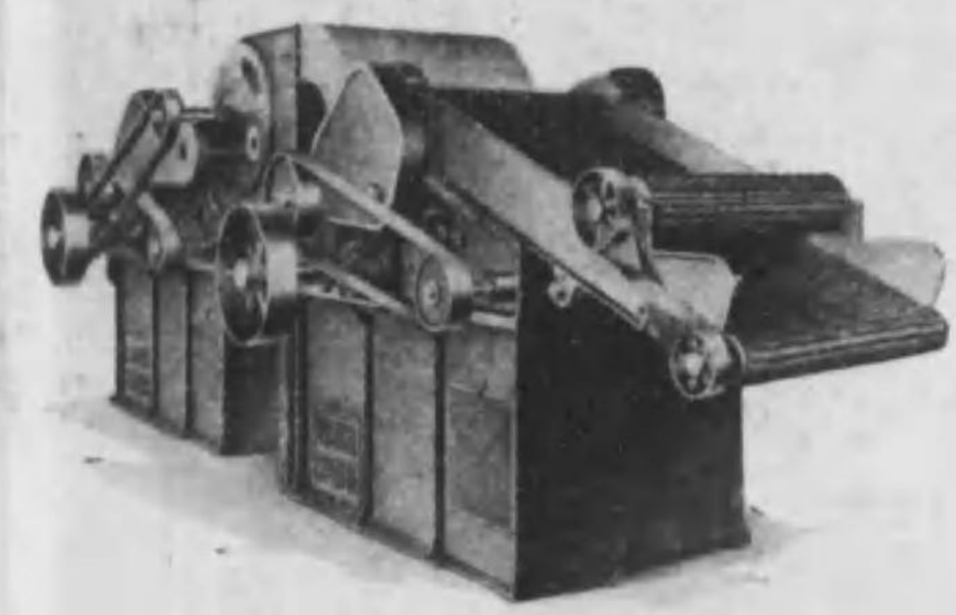
Lattice Openers in Tandem
