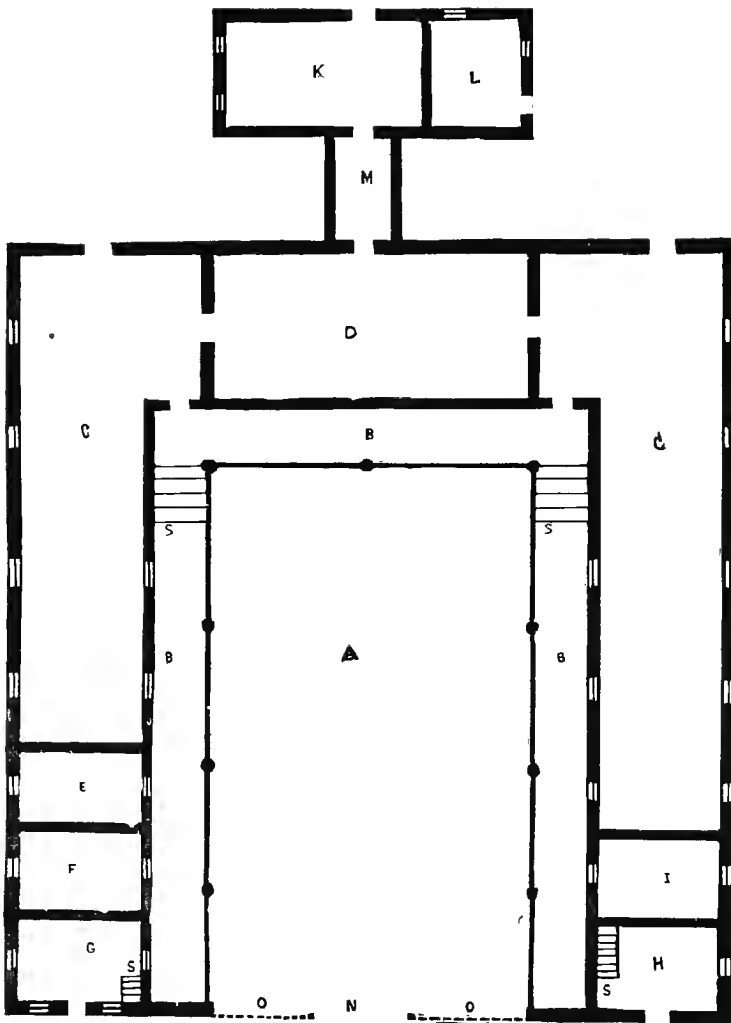
PLAN OF SOLDIERS' HOME, CAMP NELSON, KY.
