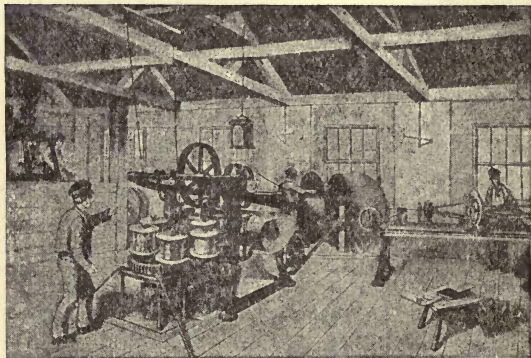
FIG. 6.—Serving the Core with Hemp-Yarn.
