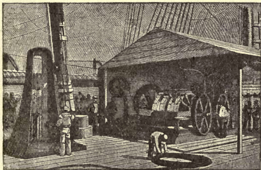
FIG. 22.—Deck of H.M.S. Agamemnon with Paying-out Apparatus.
