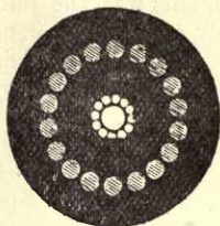
FIG. 43.—Anglo-American Atlantic Cable (1894): deep sea type.
