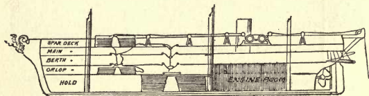
FIG. 24.—The Loading of the Agamemnon .
