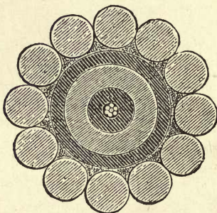
FIG. 9.—The Shore-End Cable.
