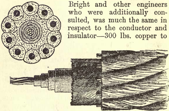
FIG. 34.—Atlantic Cable, 1865-6: Main (deep sea) Type.
