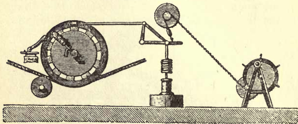
FIG. 17.—The Principle of the Brake.
