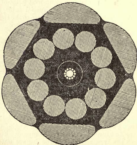
FIG. 44.—Shore end of the 1894 "Anglo" Cable.
