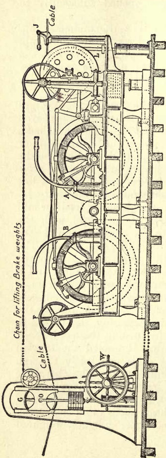
FIG. 18.—Bright's Paying-out Gear, 1858.
