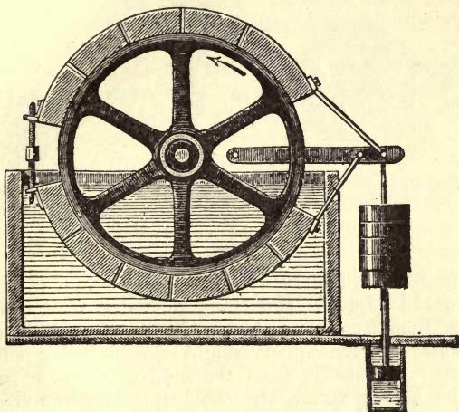
FIG. 16.—The Self-Releasing Brake.
