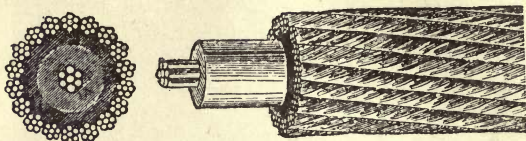
FIG. 8.—The Deep Sea Cable.
