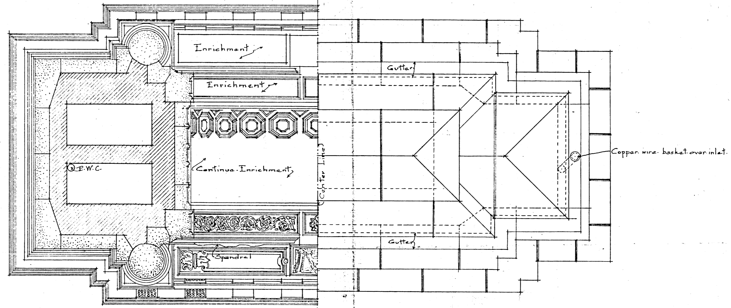
HALF PLAN AT LEVEL OF CENTER OF ARCH. HALF PLAN OF ROOF. LOOKING UP.
