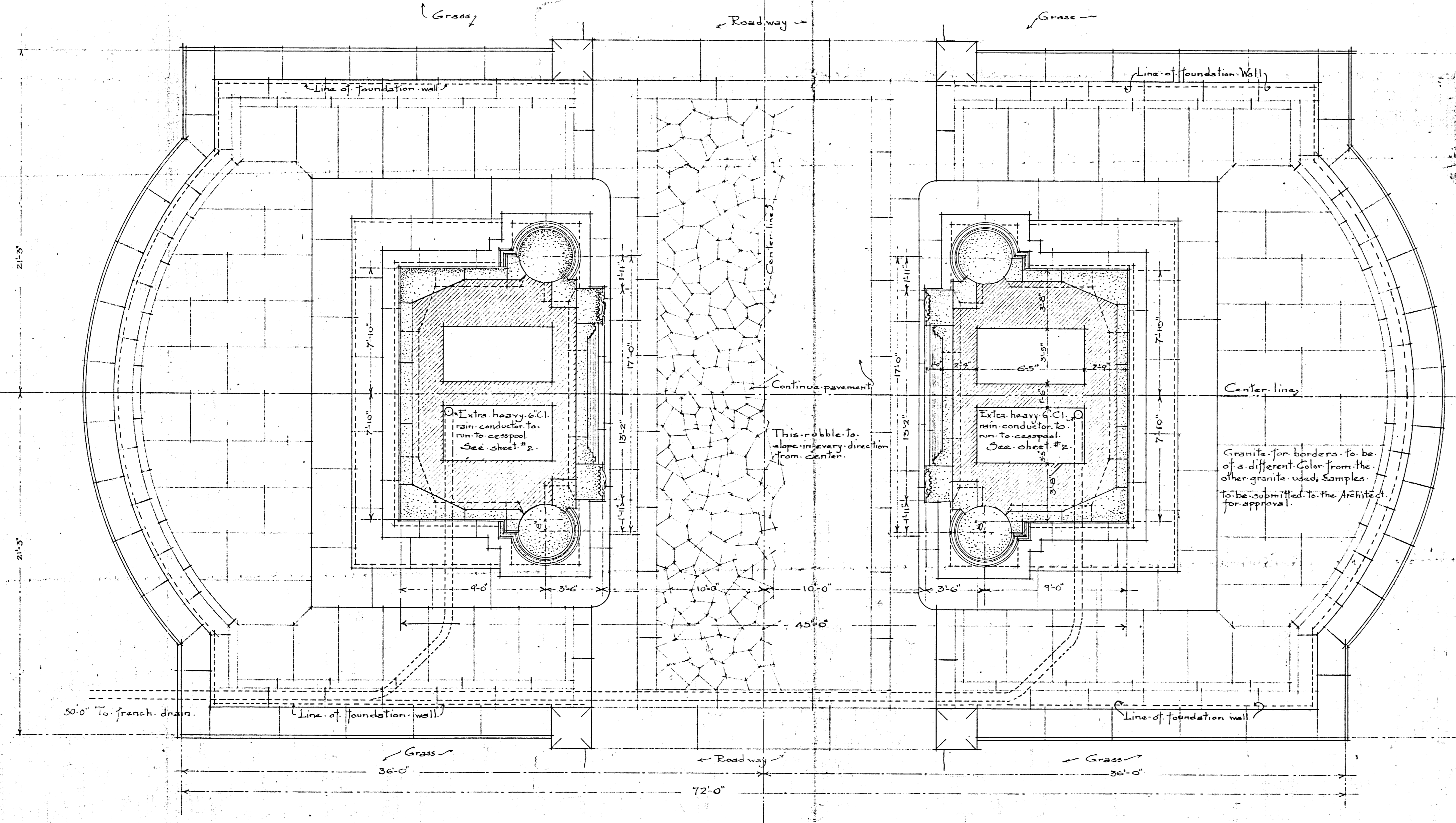
PLAN ABOVE BASE COURSE.
