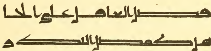
CUFIC CHARACTERS.
