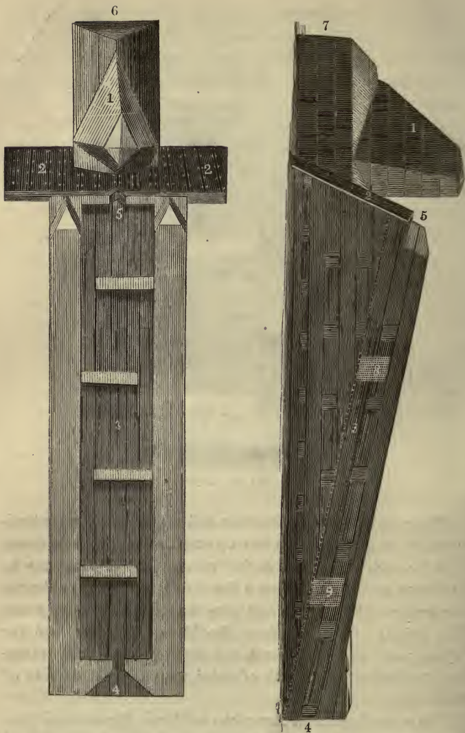
CANADIAN SALMON-STAIRS.
