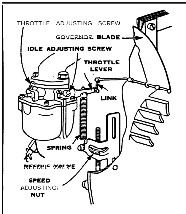
Figure 3-14. Carburetor and pneumatic governor.
