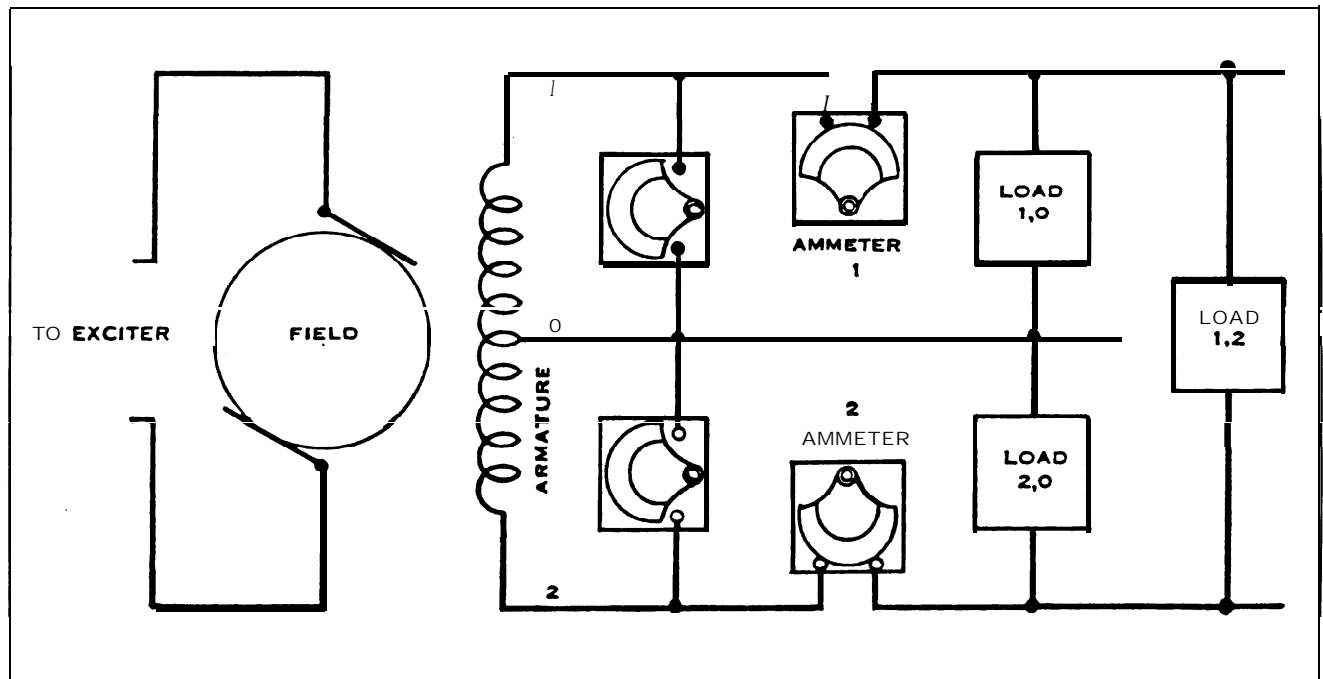
Figure 4-6. Three-wire, single-phase alternator.
