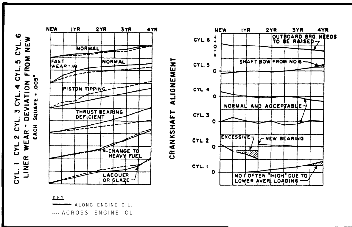
Figure 3-18. Maintenance data plots. A) 'AS-FOUND' PRESSURES, B) MEASUREMENTS OF MECHANICAL WEAR INDICATORS.
