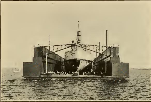
FLOATING DRY DOCK DEWEY
