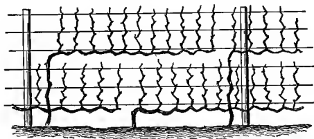
FIG. 76.—Thomery training.
