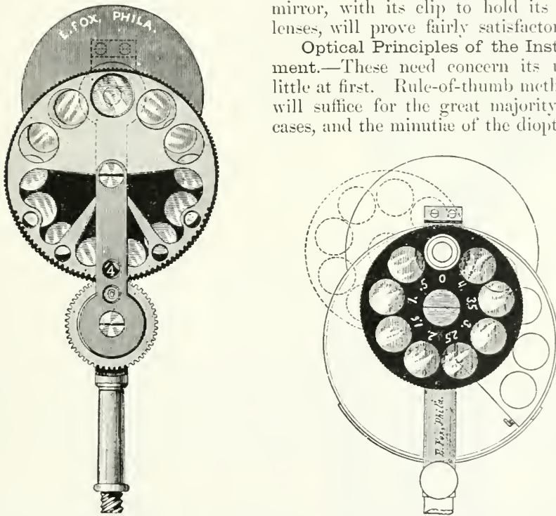
FIG. 119.—Randall's modified Loring ophthalmoscope, in which the "quadrant" is moved by the cog below, so that every glass can be brought to the sight-hole without removing the instrument from the eye. A disk of concave cylinders 0.5 to 4, is eccentrically mounted, so that each can be brought at any desired inclination of its axis into combination with any spherical. It gives 51 spherical lenses or combinations. The mirror can be detached to substitute a weak-light, plane, or more concave mirror, or left off, uncovering the 6 mm. breadth of the lenses when the instrument is used as an optometer. The disk of cylinders can be left off as drawn, or attached to any form of ophthalmoscope.
