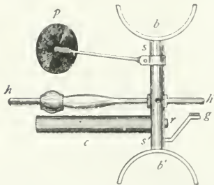
FIG. 470.—Poltzer acoumeter, with the steel rod c to be struck by the hammer h falling just the distance permitted by the stop g , while the thumb and index finger grasp it at bb' , and can rest the disk p against the bone of the head.
