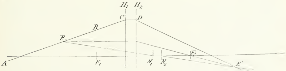
FIG. 51.—Diagram to find the refracted ray in the last medium of a given ray in the first medium.
