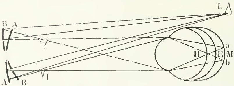
FIG. 155.—Course of rays in skiascopy with concave mirror: A A, one position of mirror giving immediate source of light at l , and illuminating retina toward a ; B B, another position of mirror with immediate source of light at l' , and retina illuminated toward b .
