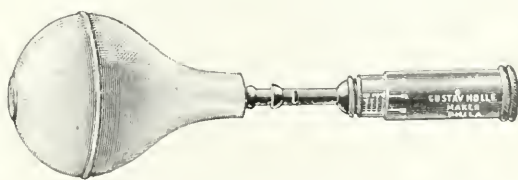
FIG. 472.—Galton's whistle with rubber bulb. The pipe below the opening is filled by a plunger advanced or withdrawn by a screw, each turn being shown by the scale upon the enlarged tube, and its tenths by that on the revolving collar. It gives an audible sound from 0.5 (theoretically, 81,000 v. s.) to 10 or 12 (4200 or 2500).
