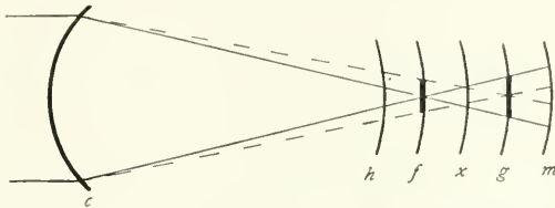
FIG. 163.—Figure illustrating varieties of astigmatism.
