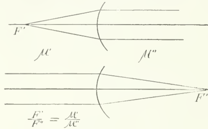
FIG. 78.—For a single surface the convergence produced in parallel rays is greater on the side of the lesser index.
