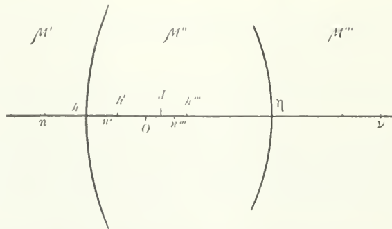
FIG. 74.—The cardinal points of a three-index system: Above, h and n , first and last surfaces; h' and h''' , first and last principal points; J , middle image. Below, r and r'' , first and last centers; n' and n'' , first and last nodal points; O , optical center.
