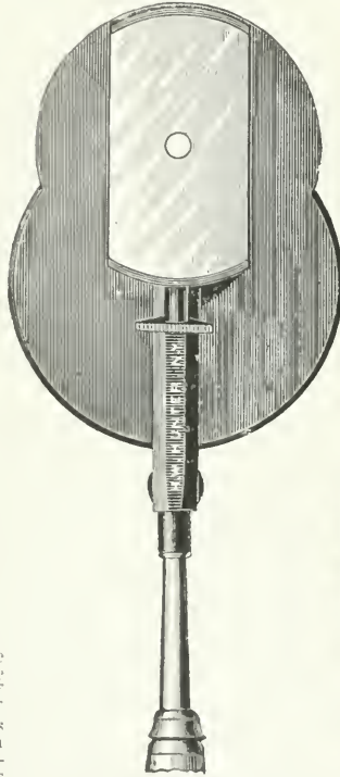
FIG. 118.—Loring's ophthalmoscope, with tilting mirror, complete disk of lenses from -1 to -8 and 0 to +7 , and supplemental quadrant containing +0.5 and +16 D. This affords 66 glasses or combinations from +23 to -21 D.
