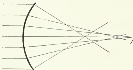
FIG. 164.—Figure illustrating spherical aberration.
