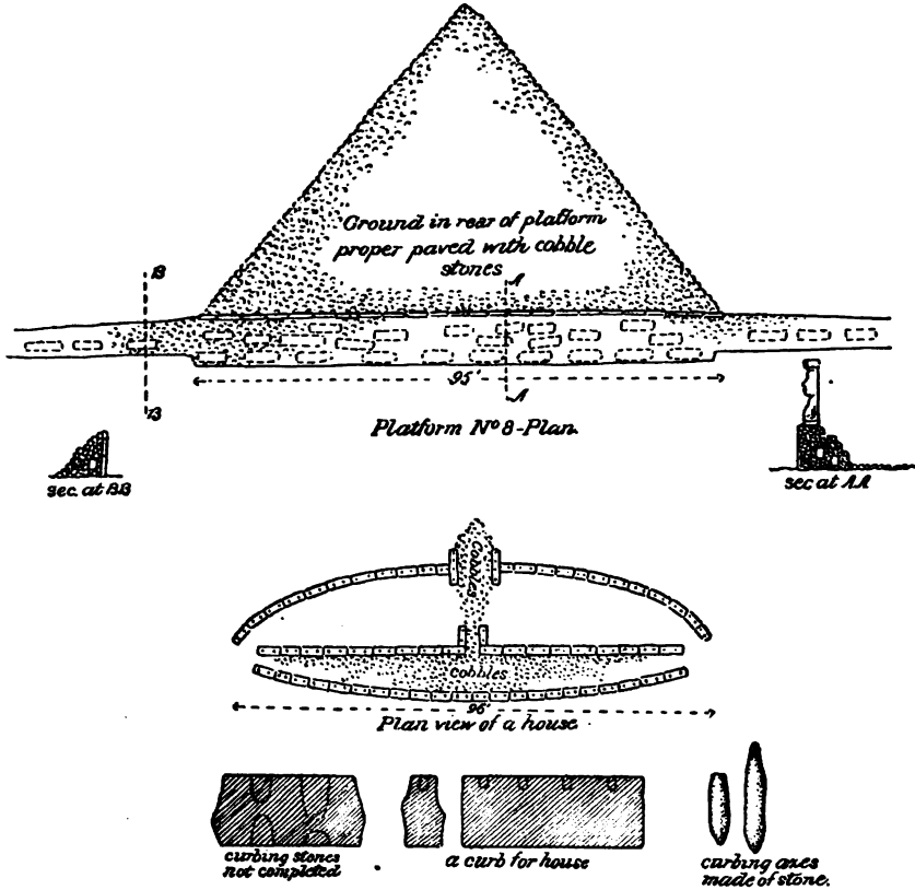
FIG. 18. SHOWING GENERAL PLAN OF CONSTRUCTION OF PLATFORM. ALSO PLAN OF HOUSE CONSTRUCTION WITH DETAILS.
