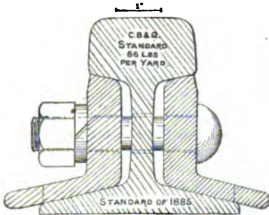
Fig. 127. ANGLE SPLICE BAR, CHICAGO, BURLINGTON AND QUINCY RAILROAD, 66-LB. RAIL, 1885. (From a drawing in the U. S. National Museum.)
