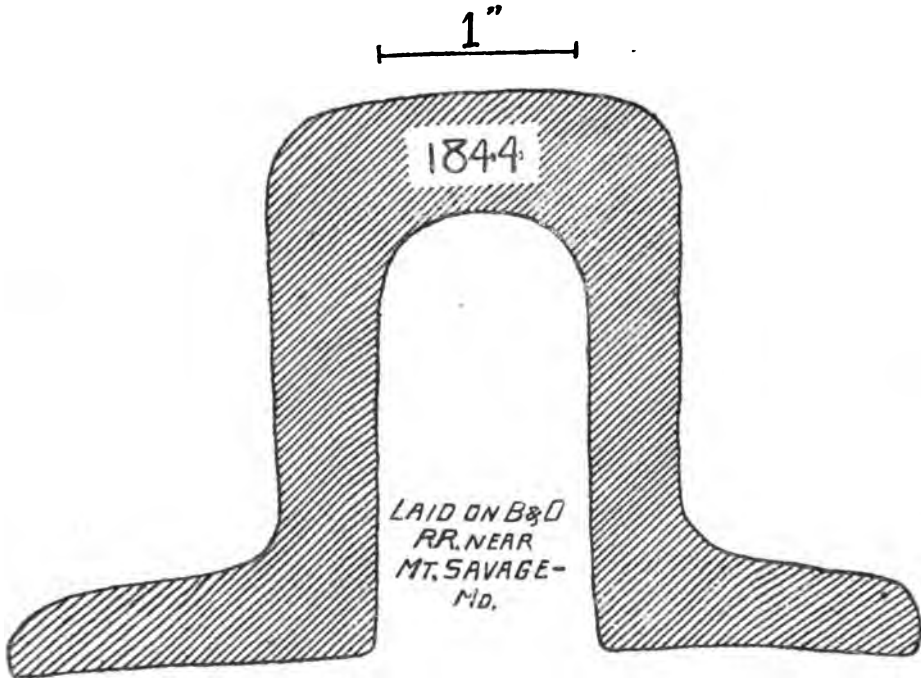
-FIRST RAIL ROLLED IN AMERICA-
