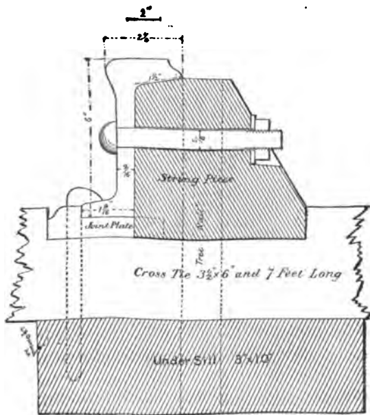
Fig. 55. COMPOUND RAIL, WOOD AND IRON. DESIGNED BY B. H. LATROBE, 1841, FOR BALTIMORE AND OHIO RAILROAD. (From a drawing in the U. S. National Museum.)
