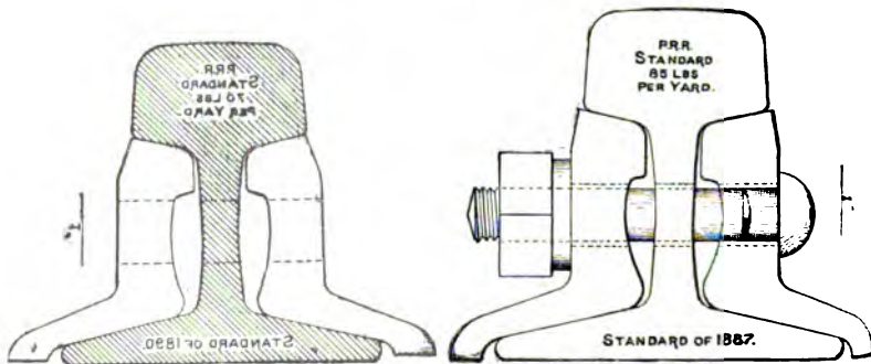
Fig. 123. ANGLE SPLICE BAR, PENNSYLVANIA RAILROAD, STANDARD FOR 70-LB. RAIL, 1890. (From a drawing in the U. S. National Museum.)
