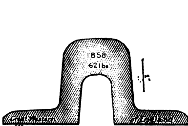
Fig. 65. "BOX RAIL," GREAT WESTERN RAILWAY OF ENGLAND, 1858. (From a drawing in the U. S. National Museum.)
