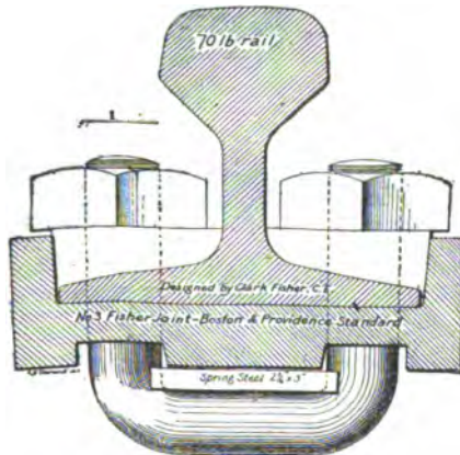
Fig. 131. FISHER & NORRIS JOINT FIXTURE AS IMPROVED BY CLARK FISHER, 1888. (From a drawing in the U. S. National Museum.)
