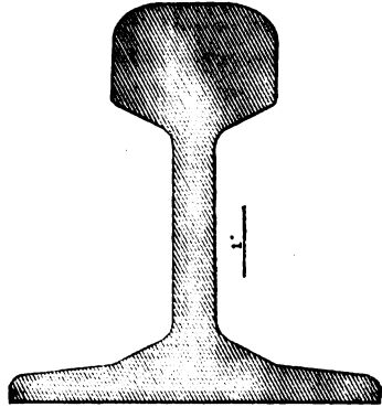
Fig. 90. STEVENS RAIL, CHEMIN DE FER DU NORD, FRANCE, 1888. (CALLED THE VIGNOLE RAIL IN EUROPE). From a drawing in the U. S. National Museum.
