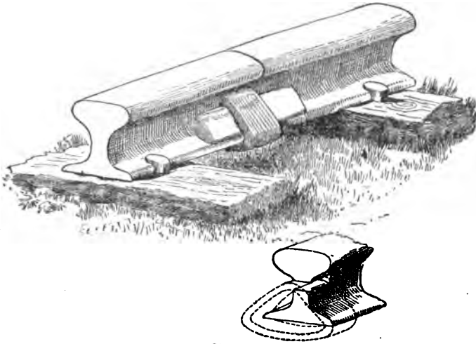
Fig. 120. RING, JOINT, AND WEDGE USED ON THE WEST JERSEY RAILROAD. (From original in the U. S. National Museum.)
