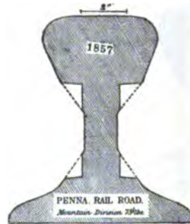
Fig. 53. 73-POUND RAIL, PENNSYLVANIA RAILROAD, MOUNTAIN DIVISION. UNDER HEAD PLANED FOR SPLICE, 1857. (From a drawing in the U. S. National Museum.)
