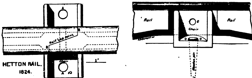
Fig. 12. HALF-LAP JOINT, HETTON RAIL, 1824. (From a drawing in the U. S. National Museum.)
