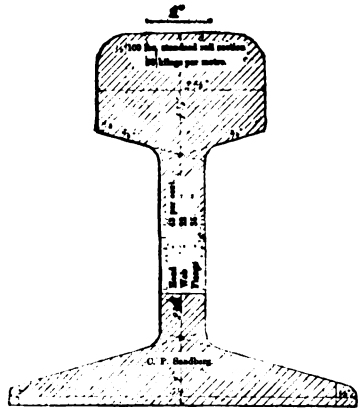
Fig. 91. STANDARD RAIL OF BELGIAN GOVERNMENT RAILWAYS, 1889. SANDBERG SECTION. From a drawing in the U. S. National Museum.
