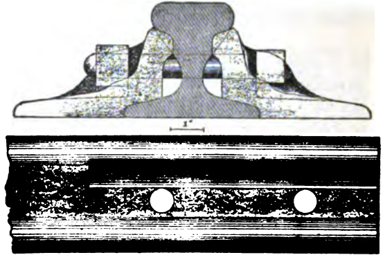
Fig. 52. ERIE RAIL WITH ENDS STAMPED FOR ADAMS' CAST-IRON BRACKET SPLICE, 1857. (From a drawing in the U. S. National Museum.)
