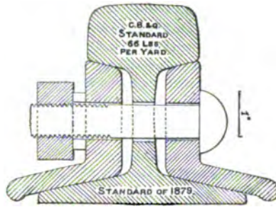
Fig. 126. ANGLE SPLICE BAR, CHICAGO, BURLINGTON AND QUINCY RAILROAD, 66-LB. RAIL, 1879. (From a drawing in the U. S. National Museum.)
