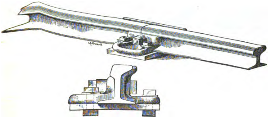
Fig. 130. JOINT FIXTURE USED ON WESTERN RAILROADS, 1869. (From original in the U. S. National Museum.)
