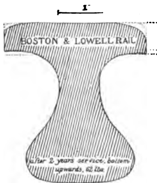
Fig. 54. 62-POUND PEAR-HEADED RAIL, BOSTON AND LOWELL RAILROAD. SHOWING WEAR AFTER TWO YEARS SERVICE, BOTTOM UPWARD. (From a drawing in the U. S. National Museum.)
