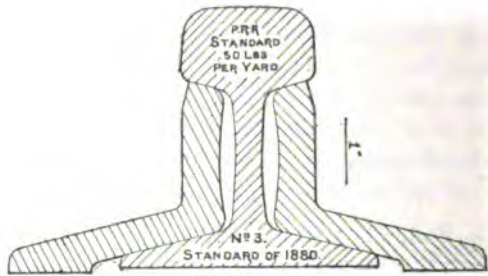
Fig. 122. ANGLE SPLICE BAR, PENNSYLVANIA RAILROAD—50-LB. RAIL, 1880. (From a drawing in the U. S. National Museum.)
