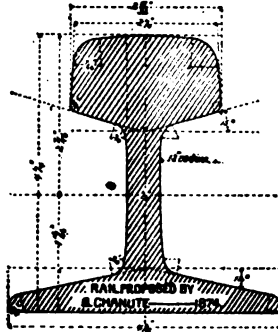
Fig. 64. RAIL PROPOSED BY O. CHANUTE, 1874. (From a drawing in the U. S. National Museum.)
