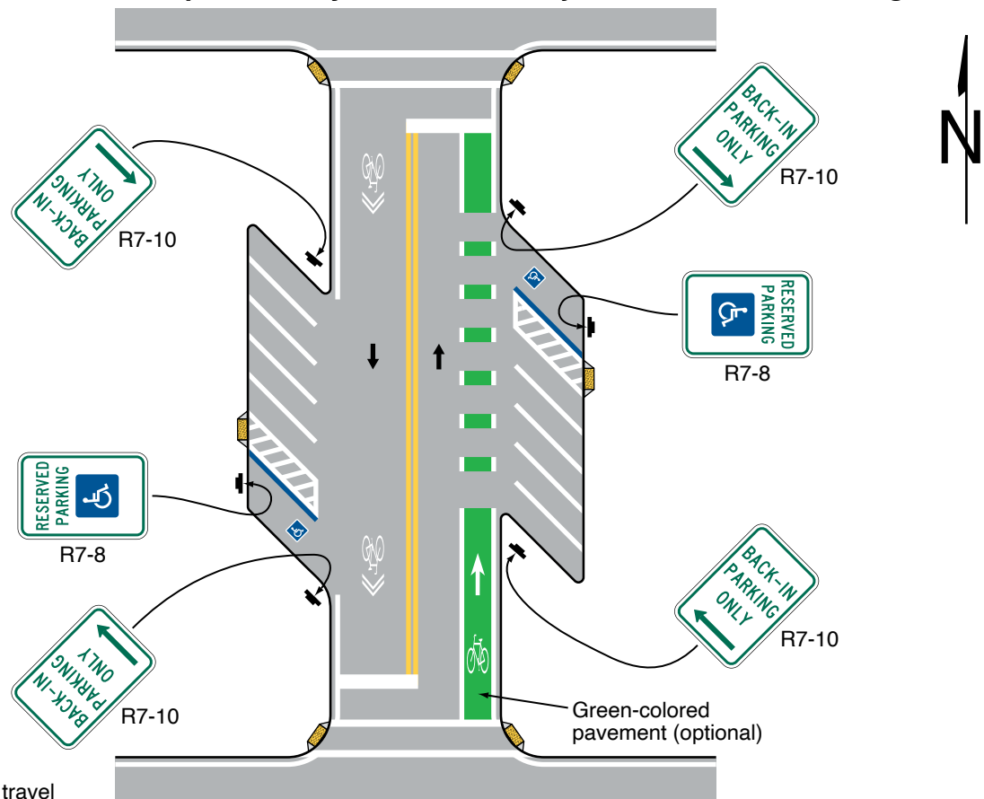
Figure 9B-3. Examples of Bicycle Facilities Adjacent to Back-In Parking
