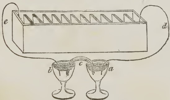
Instances of chemical decomposition by the Voltaic Battery.
