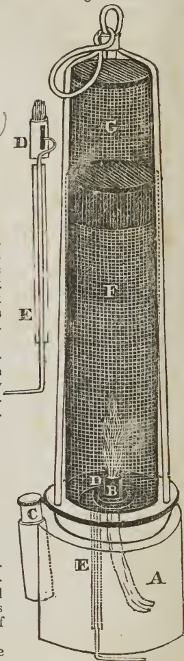
A. the cistern containing the oil. B. the rim or screw by which the gauze cage is fixed to the cistern. C. aperture for supplying oil. E. a wire for trimming the wick D. F. the wire gauze cylinder. G. a double top.
