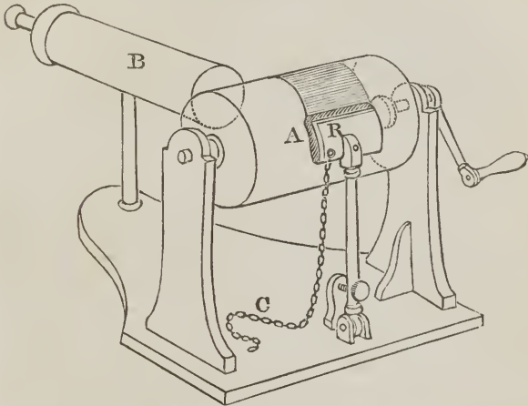
Fig. 13. A the Cylinder. B the Conductor. R the Rubber. C the Chain.
