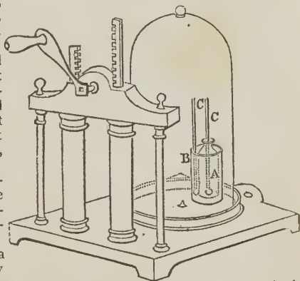
Fig. 7. Pneumatic Pump.
