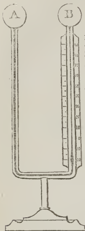
Fig. 4. Differential Ther- mometer.
