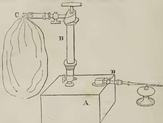
A, the reservoir of condensed air. B, the condensing syringe. C, the bladder for oxygen. D, the moveable jet.
