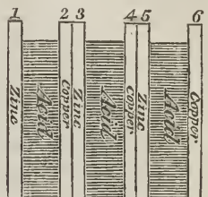
Fig. 14. Voltaic Battery.
