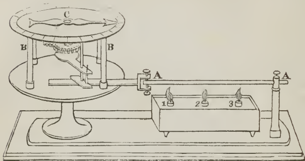
A A, Bar of metal. 1 2 3, Lamps burning. B B, Wheel work. C, Index.
