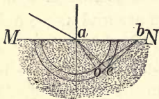
Double refraction. First case.
