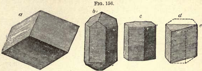
Crystalline forms of Iceland spar.
