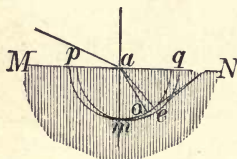
Double refraction. Third case.
