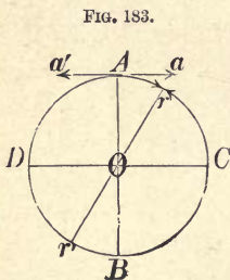
Combined effect of two opposite circular vibrations.
