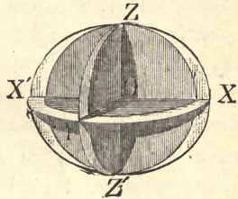
Wave-surface of a negative uniaxial crystal.
