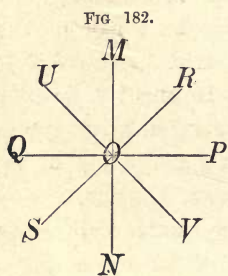
Decomposition of vibrations.
