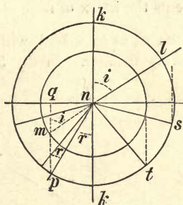
Construction of the refracted ray.
