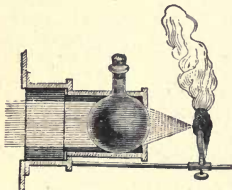
Action of the invisible thermotic rays.
