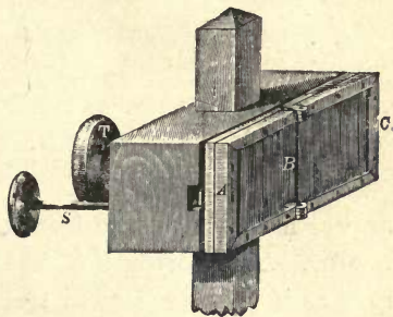
Fresnel's mirror.
