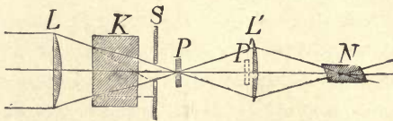
Polarising apparatus of Dubosq.
