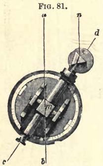
Instrument for measuring the prismatic deflection.
