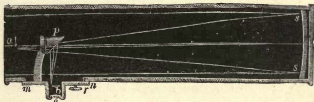
Action of Newton's reflecting telescope.
