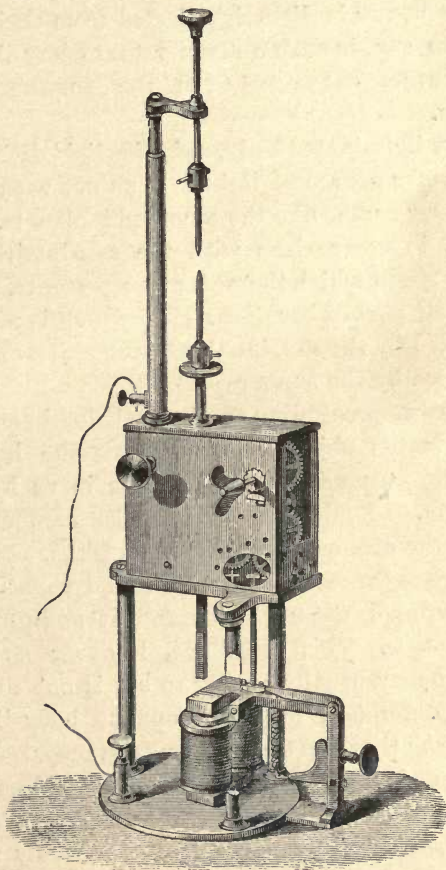
Electric lamp.
