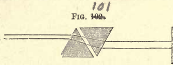
Combination of a crown and of a flint-glass prism causing dispersion but no deflection.
