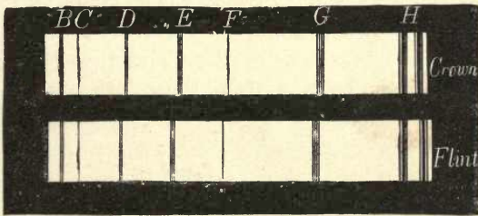
Spectrum thrown by crown glass and by flint glass.
