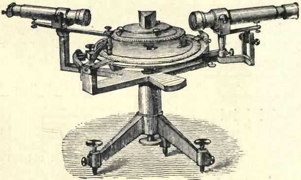
Spectrometer.
