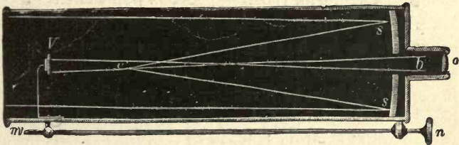
Action of Gregory's reflector.
