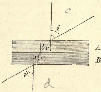
Refraction through two parallel plates.
