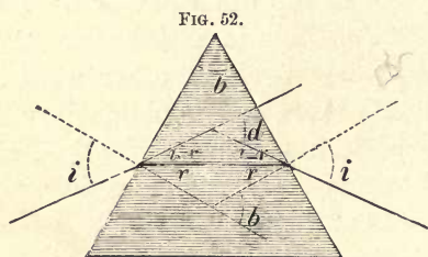
Smallest deflection through a prism.
