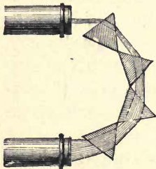
Telescopes with four prisms.
