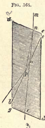
Nicol's prism.
