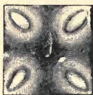
Polarisation image obtained from a suddenly cooled plate of glass.
