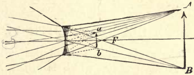
Virtual image formed by a concave lens.
