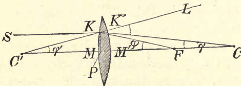
Determination of the focal distance.
