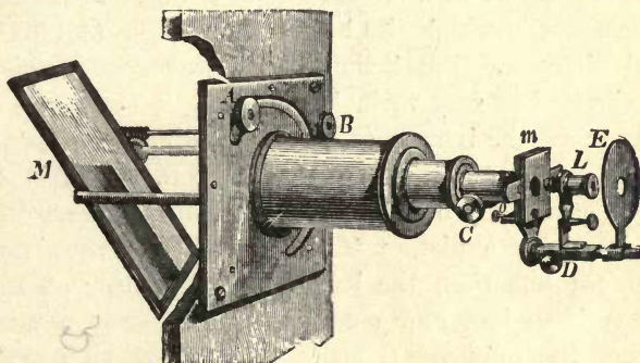
Solar Microscope.
