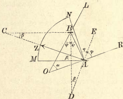
Principle of the mirror sextant .
