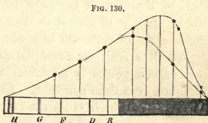
Heat-curves of the spectra thrown by flint glass and rock salt.
