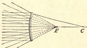
Virtual principal focus of a convex mirror.
