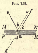
Explanation of the colours of the laminae.
