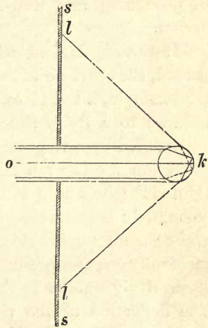
Refraction and internal reflexion in a rain-drop.
