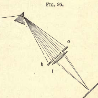
Combination of two homogeneous colours.
