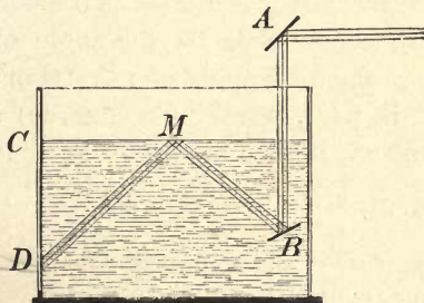
Total reflexion.
