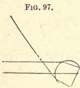
Refraction and double internal reflexion in a rain-drop.
