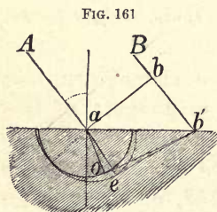
Huyghens' construction of double refraction.
