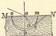
Double refraction. Second case.
