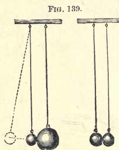
Impact of elastic balls.
