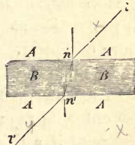
Refraction through a transparent plate with parallel surfaces.
