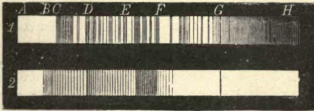
Absorption spectra of nitrous oxide and of the vapour of iodine.
