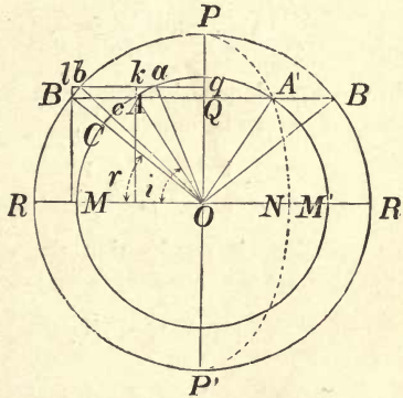
Theory of the rainbow.
