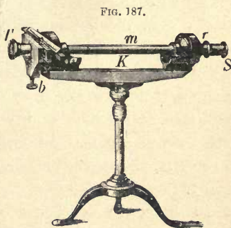
Soleil's Saccharimeter.
