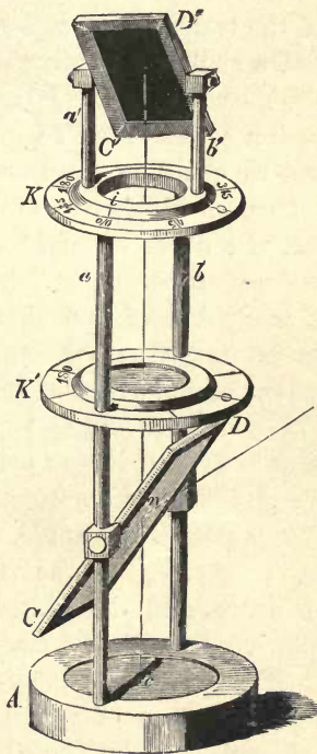
Nörremberg's polarising apparatus.
