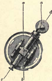
Measurement of refraction as practised by Fraunhofer.
