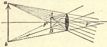
Virtual image with a convex lens.
