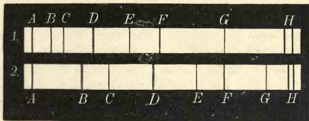
Comparison of the prismatic with the grating spectrum.
