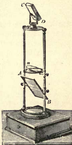
Nörremberg's polarising apparatus with glass laminae.
