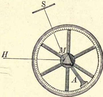
Principle of the Reflecting Goniometer.
