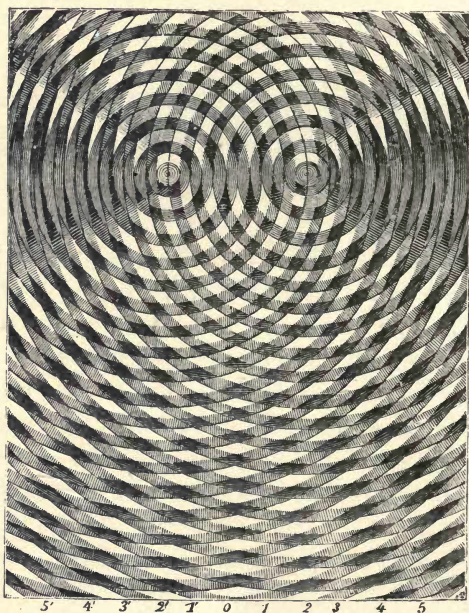
Interference of two systems of waves.
