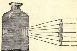
Fluorescence.
