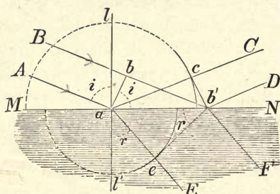
Explanation of reflexion and refraction.
