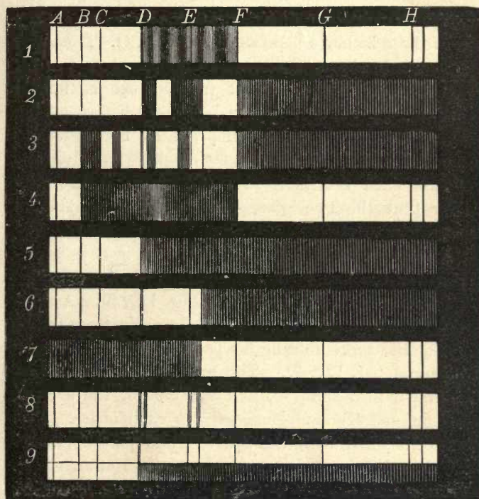
Absorption spectra.
