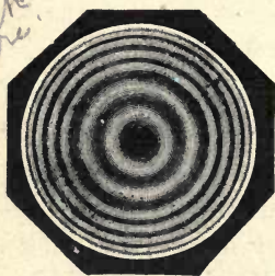
Newton's coloured rings.
