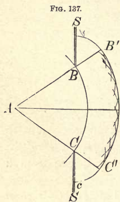
Huyghens' principle.
