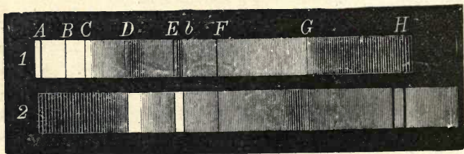
Absorption and fluorescing spectrum of Naphthalin red.
