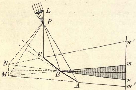
Fresnel's mirror experiment.
