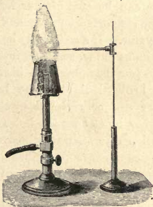
Bunsen's burner.
