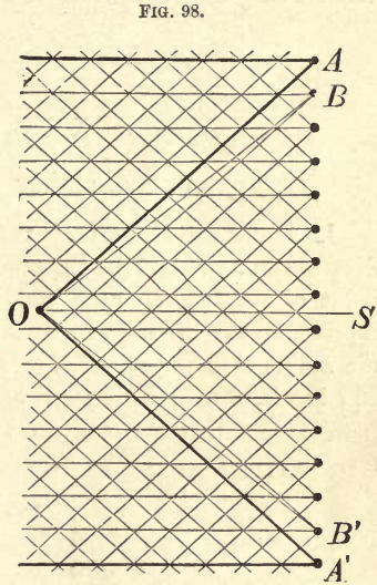
Mode of formation of the rainbow.
