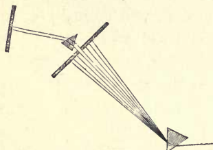
Undecomposability of the colours of the spectrum.
