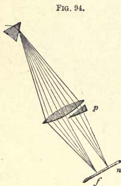
Complementary colours.
