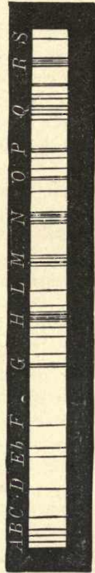
Fig. 123.—Solar spectrum with the ultra-violet portion.
