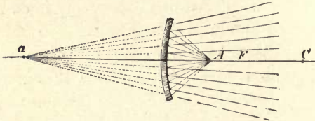
Conjugate points.
