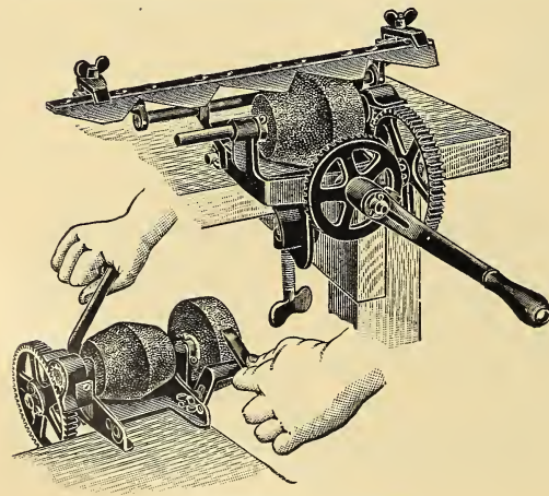
Carborundum Grinder
