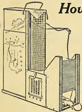
PEERLESS AUTOMATIC MOUSE TRAP
