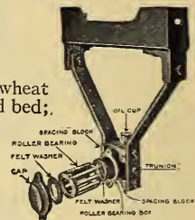
Roller-Bearing Hanger
