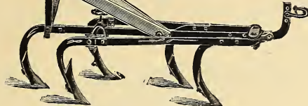
Pittsburgh 5-Tooth with Hand-Wheel Adjustment
