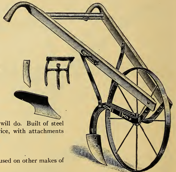
Star Garden Cultivator
