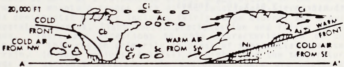
Cross Section Through a Cold Front and a Warm Front
