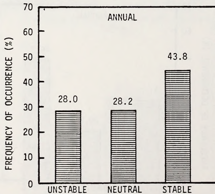
Figure 4.5-5 Seasonal/Annual Distribution of Atmospheric Stability Lovellock, Nevada (1966-1970)
