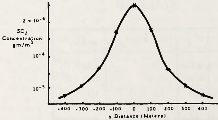
Figure 4.9-12 Concentration of SO 2 (gm/m 3 ) Across Wind at a Distance of 800 Meters (Problem 3)
