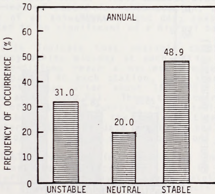
Figure 4.5-4 Seasonal/Annual Distribution of Atmospheric Stability Fallon, Nevada (1966-1970) 198
