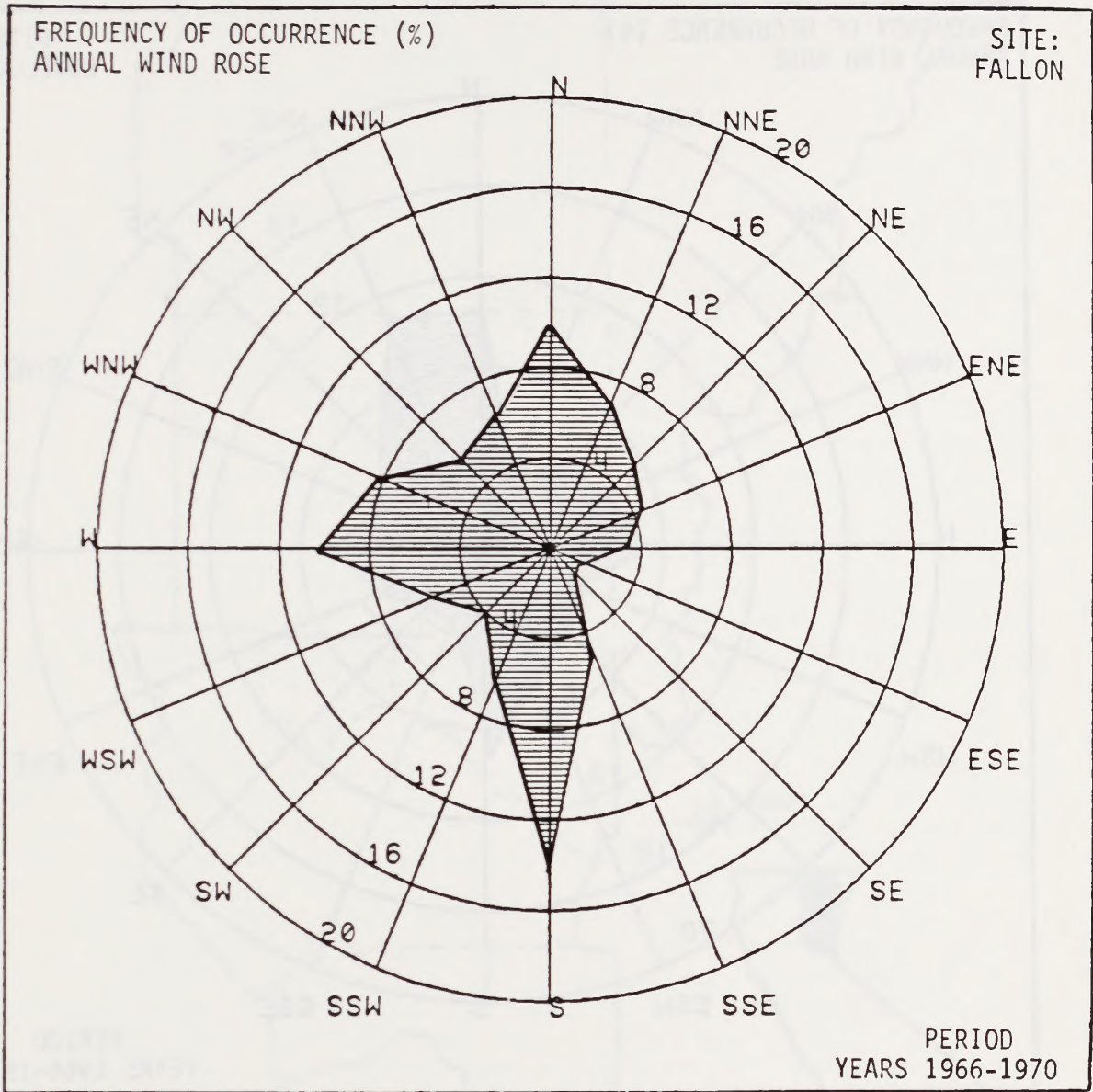
Figure 4.4-3 Annual Wind Rose for Fallon (1966 - 1970)
