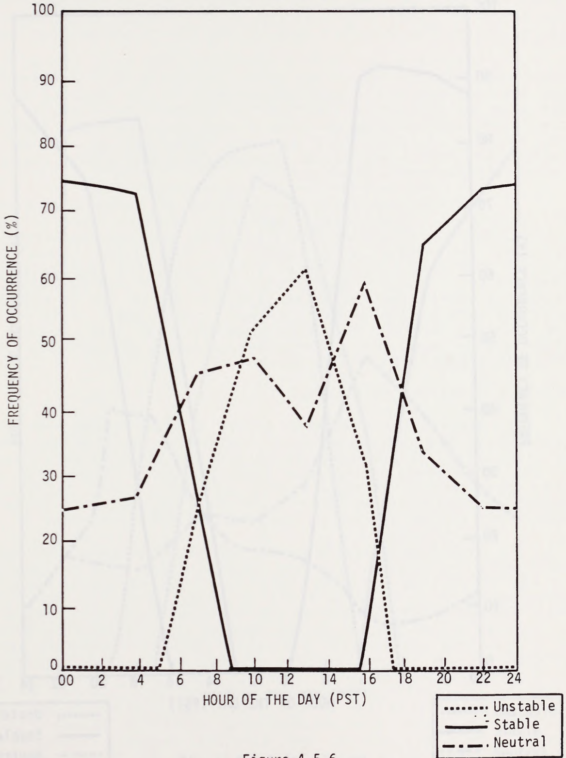
Figure 4.5-6 Diurnal Distribution of Atmospheric Stability in the Susanville District
