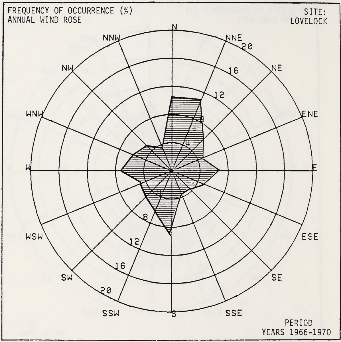
Figure 4.4-4 Annual Wind Rose for Lovelock (1966 - 1970)
