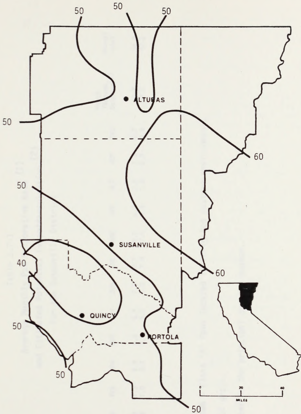
Figure 3.7-2 Annual Evaporative Demand in the Susanville District
