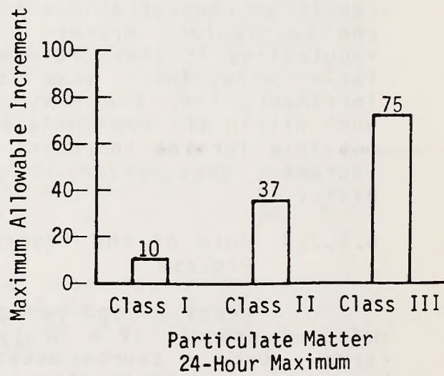
Figure 6.1-1 Prevention of Significant Deterioration Maximum Allowable Increments as a Function of Class Designation ( \mu\text{g}/\text{m}^3 )
