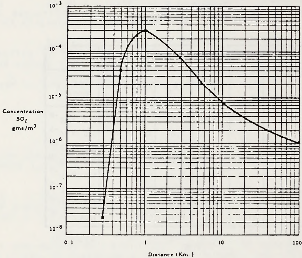
Figure 4.10-11 Concentration of SO 2 (gm/m 3 ) as a Function of Distance (km). (Problem 2)
