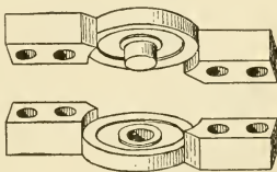
Fig. 435.—Heavy Sash Centre for Vertical Swing.
