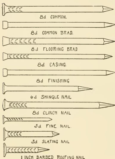
Fig. 330.—Wire Nails (Full Size).
