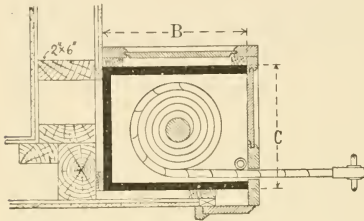
Fig 506.—Casing of Coil Box, Vertical Flexifold Partitions.
