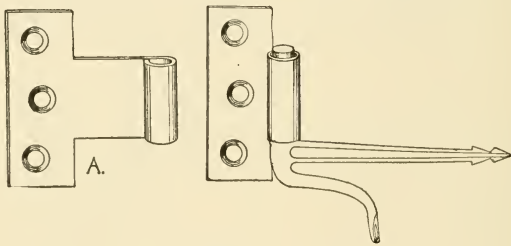
Fig. 441.—Wrought Steel Blind Hinge.
