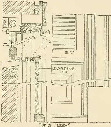
Fig. 259.—Detail for Sliding Blinds.
