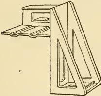
Wall Hanger for joists 6x14 and under. Self releasing, no holes in wall.
