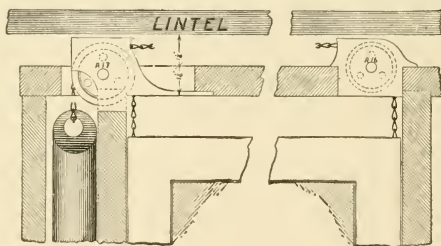
Fig. 422.—Queen Mullion Frame Pulleys.
