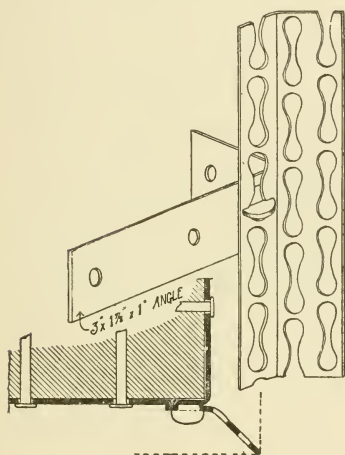
Fig. 198.—Empire Corner Plate, Half Full Size.
