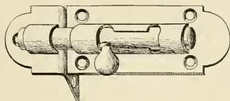
Fig. 401.—Barrel Bolt, Bent Staple.
