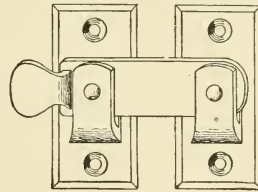
Fig. 440.—Shutter Bar.
