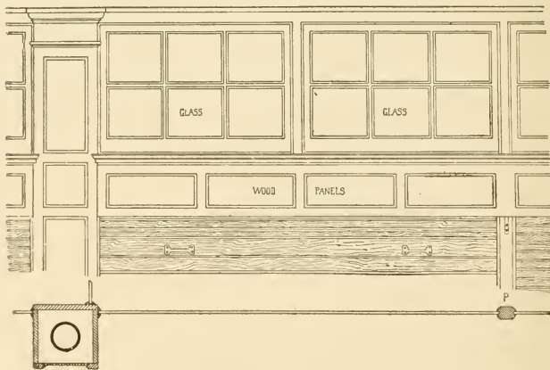
Fig. 504.—Casing for Wilson's Rolling Partitions.
