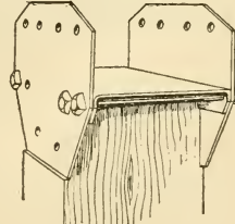
Two-way Post Cap. All steel. Three-way and four-way caps also carried in stock.
