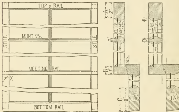
Fig. 117.—Sash Details.
