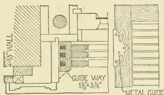
Fig. 260.—Poppert's Weight Sliding Blind.
