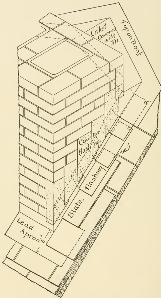
Fig. 177.—Flashing of Chimney.
