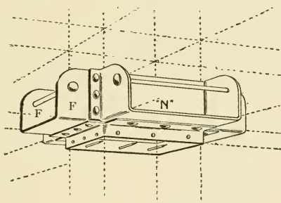
Fig. 466.—Van Dorn's Steel Post Cap.
