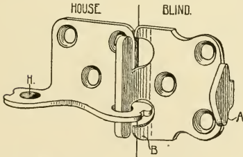
Fig. 443.—Stanley Gravity Blind Hinge.
