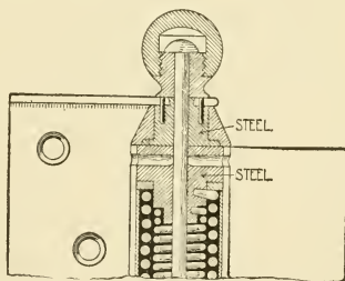
Fig. 350.—Section Through Cylinder of Bommer Hinge.
