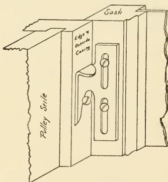
Fig. 449.—Moore's Storm Window Fastener.
