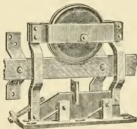
Fig. 359.—Lane Ball-Bearing Hanger.
