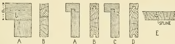
Fig. 199.—Butt Joints.
