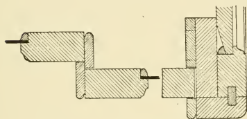
Fig. 314.—Detail of Sliding Cupboard Doors and Frame.
