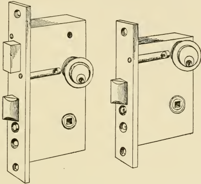
Fig. 385 — Yale Front Door Lock and Vestibule Latch.
