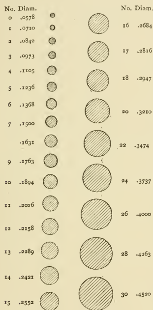
Fig. 333.—American Screw Gauge.
