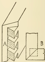
Fig. 207.—Secret Dovetail.
