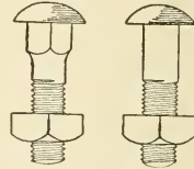
Fig. 335.—Button-Head Bolts.
