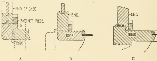
Fig. 316—Methods of Hanging Doors of Cases.
