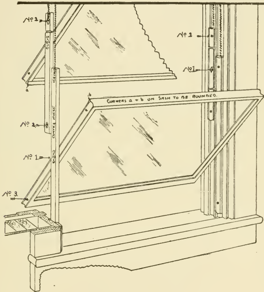
Fig. 106.—Bolles' Patent Revolving Sash.
