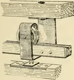
Fig. 366. Wilcox Swivel Hanger; Ball-Bearing.
