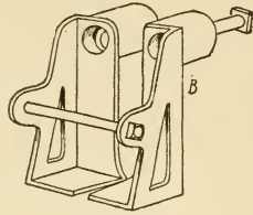
Hangers for joists over 8 ins. wide.
