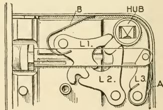
Fig. 371.—Latch of Yale "Vulcan" Lock.
