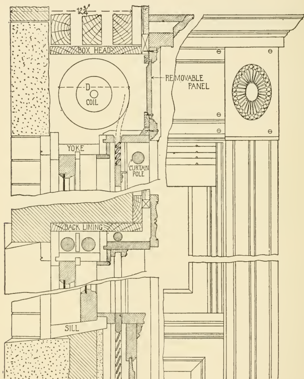
Fig. 262 —Detail for Rolling Blinds.
