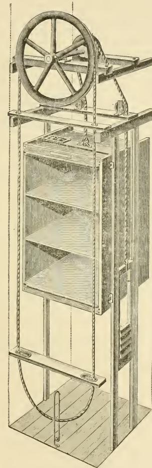
Fig. 520.—Sedgwick Automatic Dumb Waiter. (Sedgwick Machine Works)
