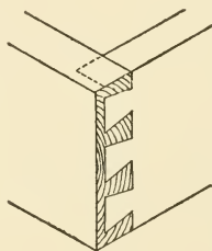
Fig. 206.—Lapped Dovetail.
