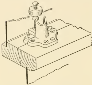
Fig. 428.—Yale Screw Sash Fast.
