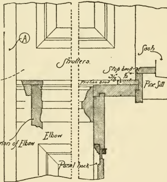
Section through window stool. ..Figure 252
