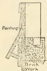
Fig. 156.—Water Table.
