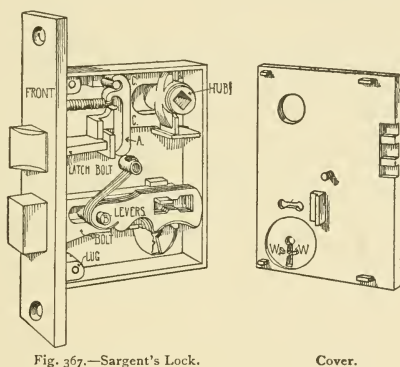
Fig. 367.—Sargent's Lock.
