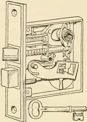
Fig. 370.—Lock and Latch.
