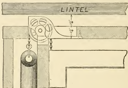
Fig. 421.—Queen Overhead Pulley.
