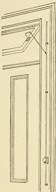
Fig. 412.—Transom Lifter.
