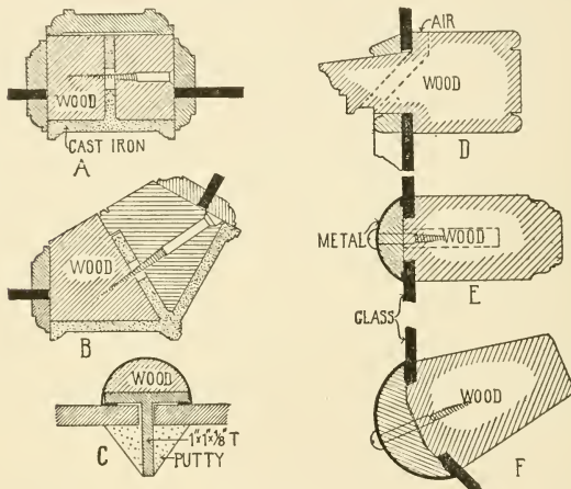
Fig. 118.—Sash Bars.
