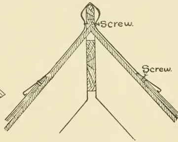
Fig. 169.—Ridge Cresting.
