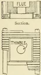
Fig. 188—Elevation.
