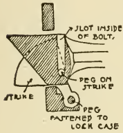
Fig. 372.—Anti-Friction Strike.
