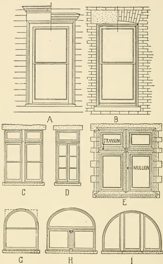
Fig. 93—Types of Windows.
