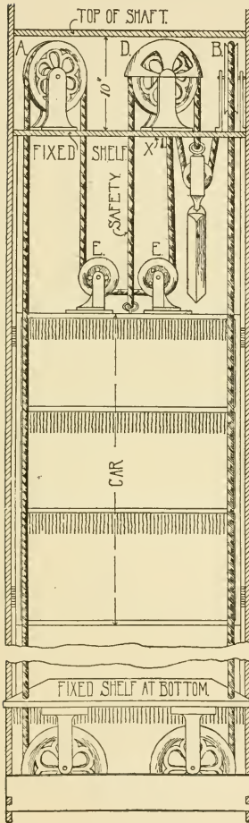
Fig. 517.—New York Safety Dumb Waiter.
