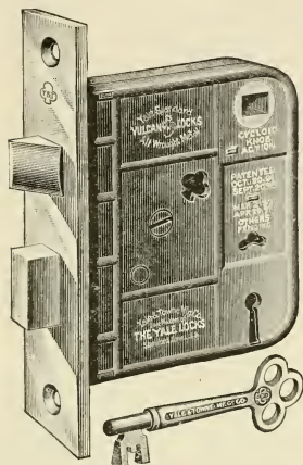
Fig. 397.—Vulcan Wrought Metal Lock.
