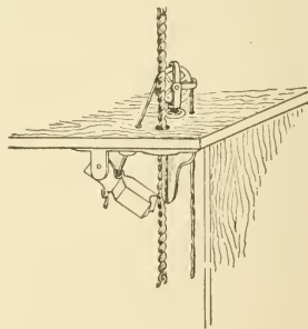
Fig. 519.—Brake Grip.
