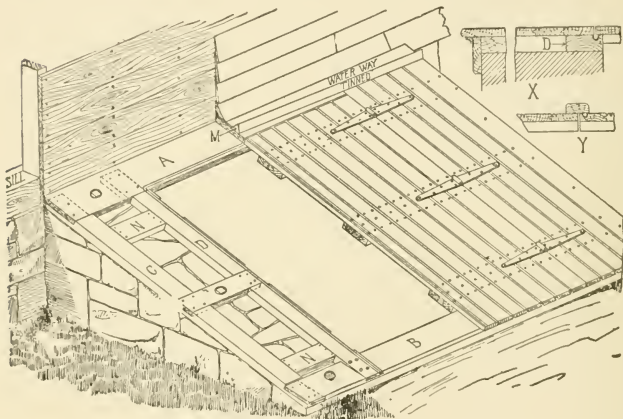
Fig. 127.—Outside Cellarway or Bulkhead.
