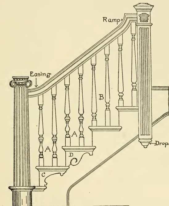
Fig. 299.—Open String.
