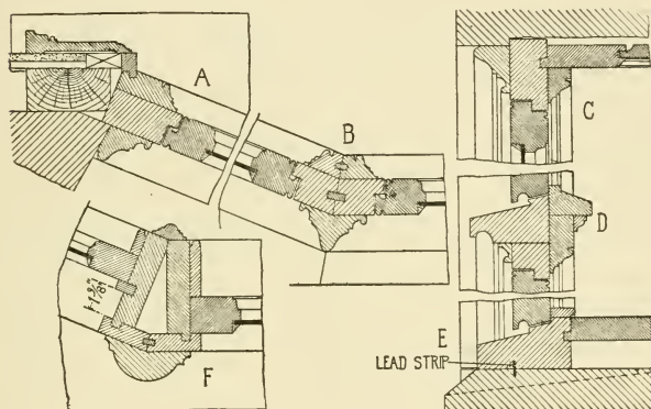
Fig. 116.—Detail of Bay Windows.
