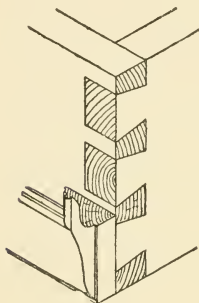
Fig. 205.—Common Dovetail.
