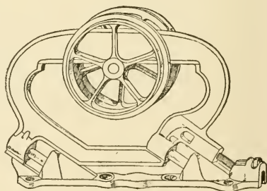
Fig. 361.—Richard's Hanger for Wood Tracks.
