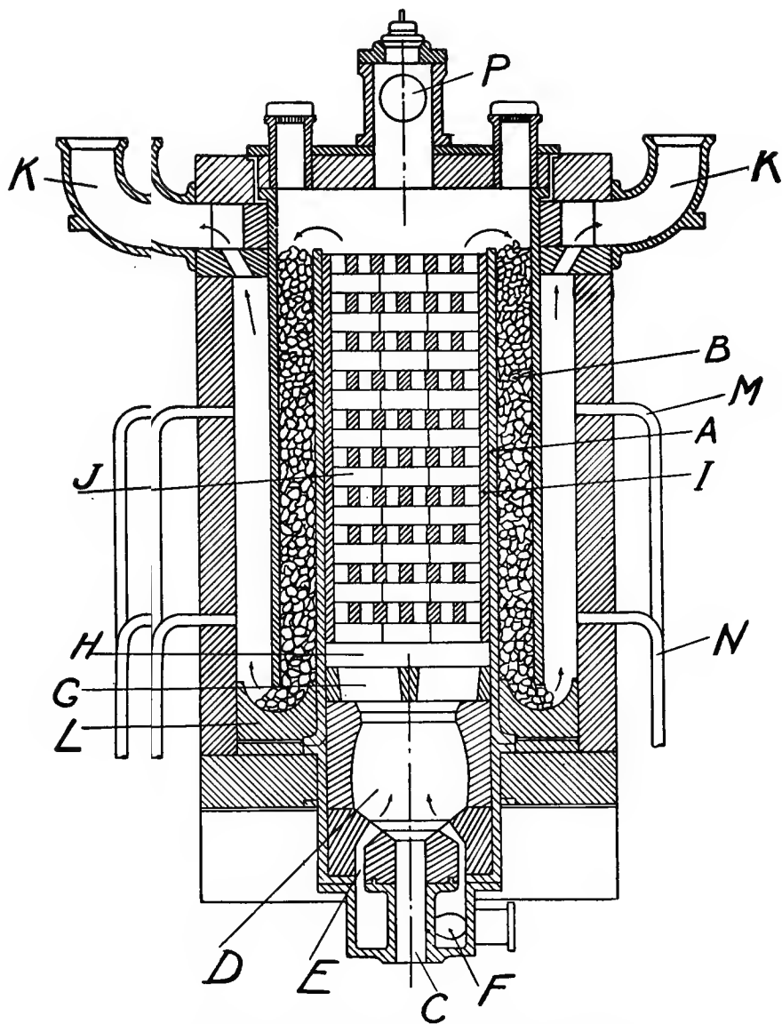
FIG. V. Single Retort Unit for Steam-Iron Process.
