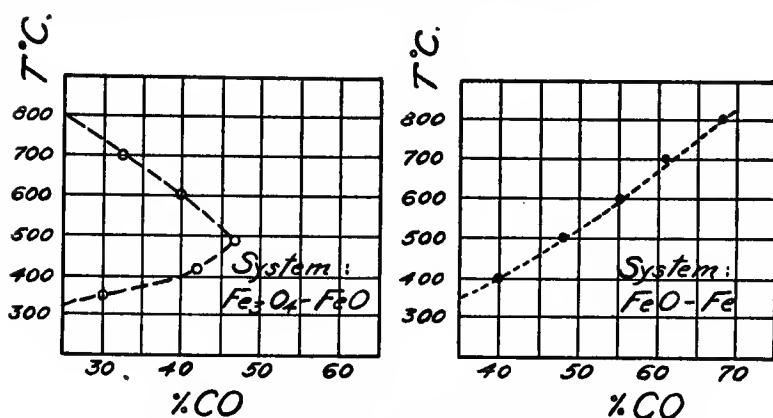
FIG. II. Fe-FeO and FeO-Fe 2 O 3 Equilibria.
