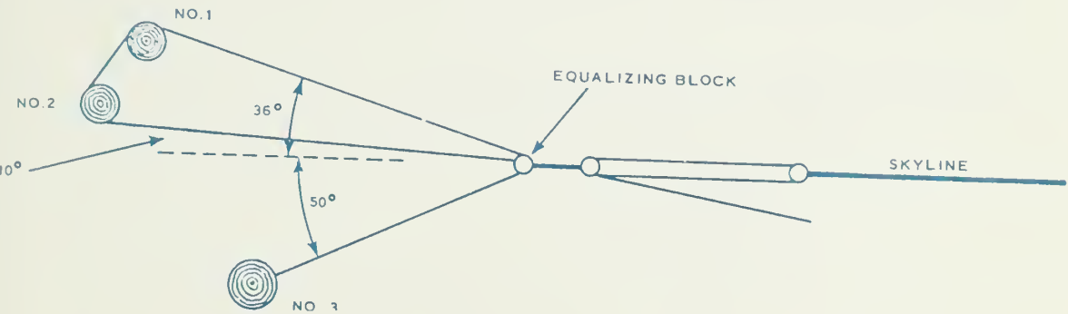
FIGURE 12a - PLAN VIEW OF STUMP ANCHOR WITH TWO STUMPS BUNDLED TOGETHER
