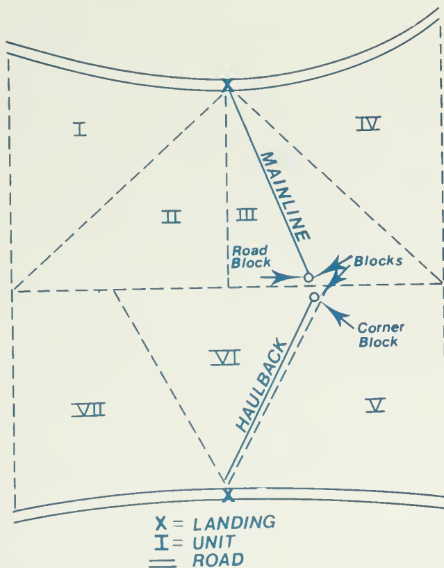
AREA PLAN SHOWING POSSIBLE YO-YO UNIT LAYOUT
