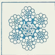
6x26 WARRINGTON-SEALE
