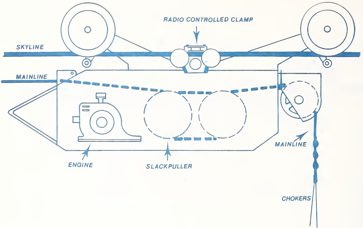
PROPANE ENGINE IN CARRIAGE PULLS SLACK OFF MAINLINE DRUM
