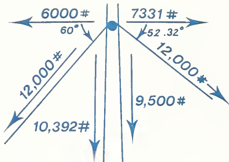
SUPPORT LINE FORCES
