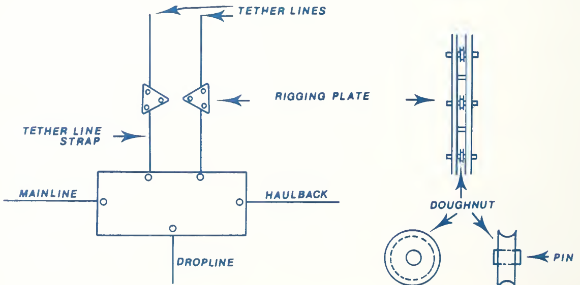
LINES USED IN BALLOON LOGGING
