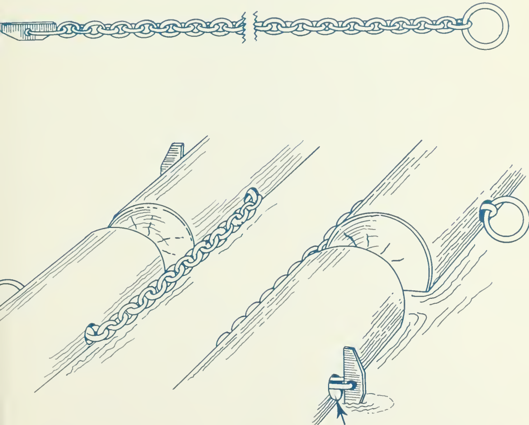
BOOM CHAIN & METHOD OF HITCHING
