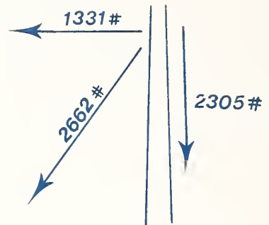
GUYLINE FORCES
