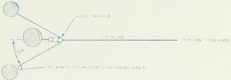
FIGURE 5a - PLAN VIEW OF TYPICAL THREE-STUMP ANCHOR
