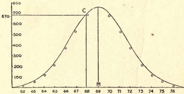
FIG. 67.—NORMAL FREQUENCY CURVE. (After Lock.)
