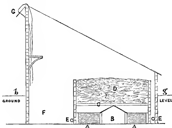
Fig. 1.—END SECTION OF CUCUMBER PIT.
