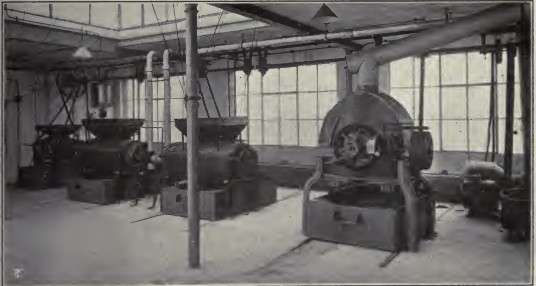
AN ENGLISH FOUR-MACHINE GAS COFFEE-ROASTING PLANT
