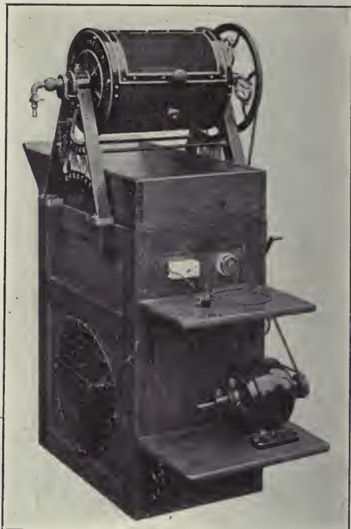
UNO CABINET GAS ROASTER WITH COOLING UNIT A popular English type
