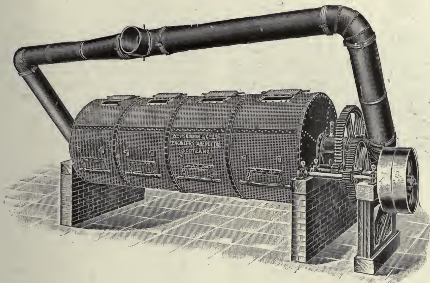
MCKINNON'S GUARDIOLA COFFEE DRIER
