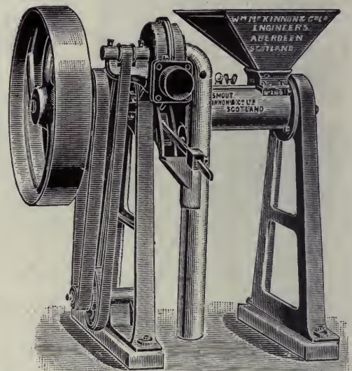
THE SMOUT PEELER AND POLISHER
