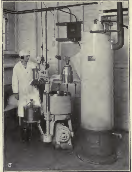
THE MANTHEY-ZORN RAPID COFFEE INFUSER AND DISPENSER
