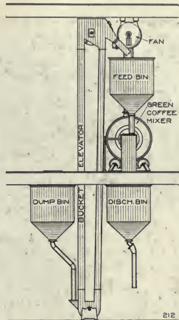
GREEN-COFFEE-MIXER CONNECTIONS
