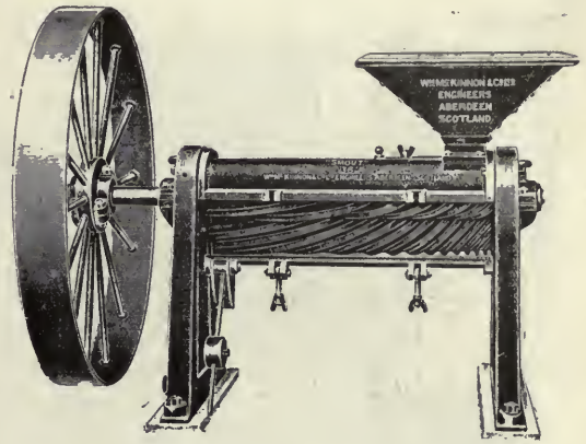
THE SMOUT PEELER AND POLISHER, WITH CYLINDER OPEN SHOWING CONE
