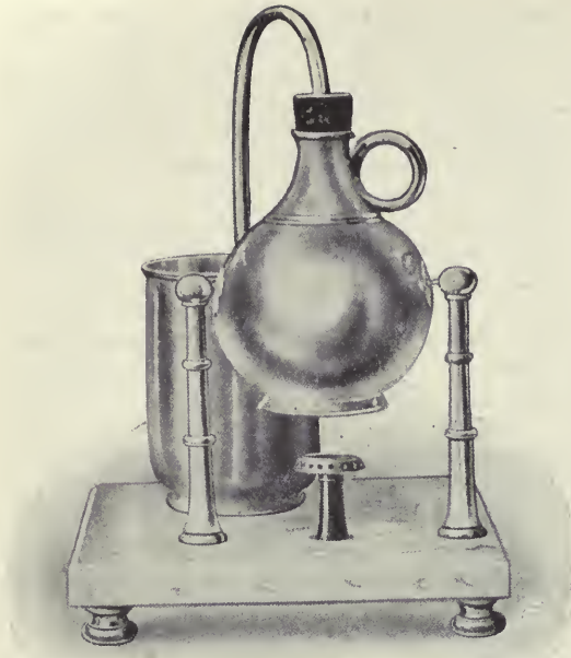
NAPIER VACUUM COFFEE MAKER
