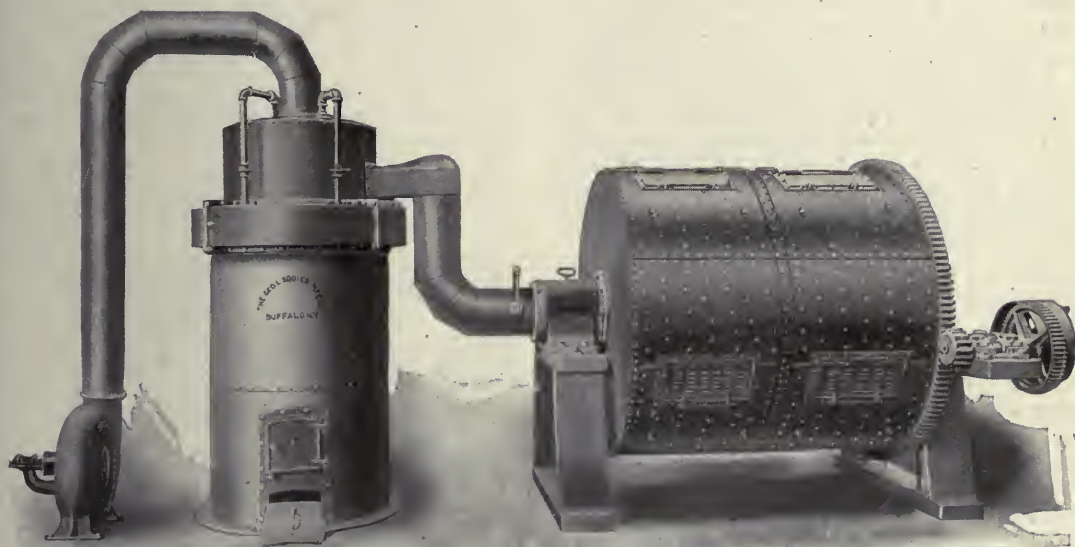
THE SQUIER-GUARDIOLA COFFEE DRIER, WITH DIRECT-FIRE HEATER
