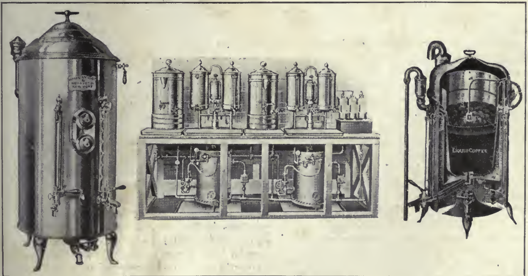
Still's machine
