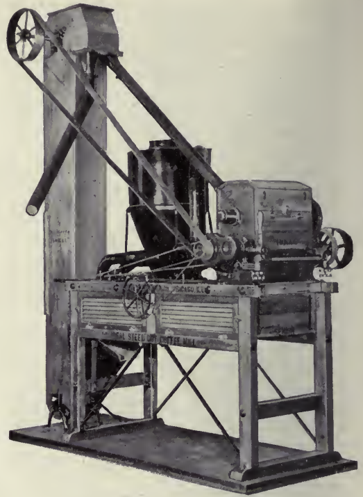
THE IDEAL STEEL-CUT MILL
