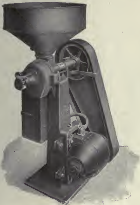
BURNS NO. 12 GRINDING MILL Designed for hotel and restaurant trade
