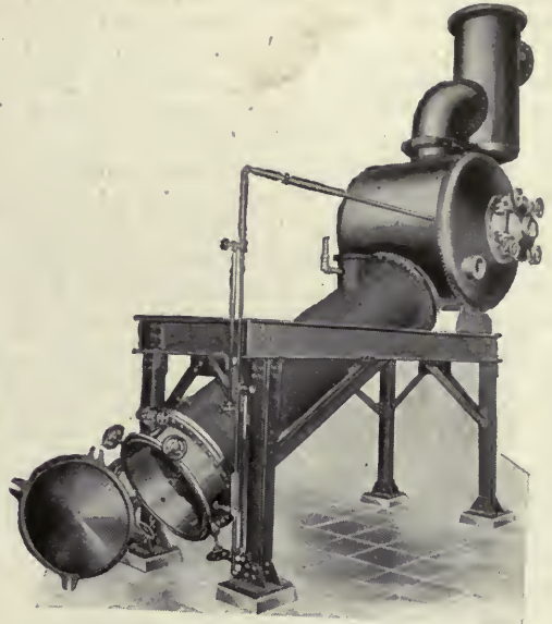
RAPID-CIRCULATION EVAPORATOR
