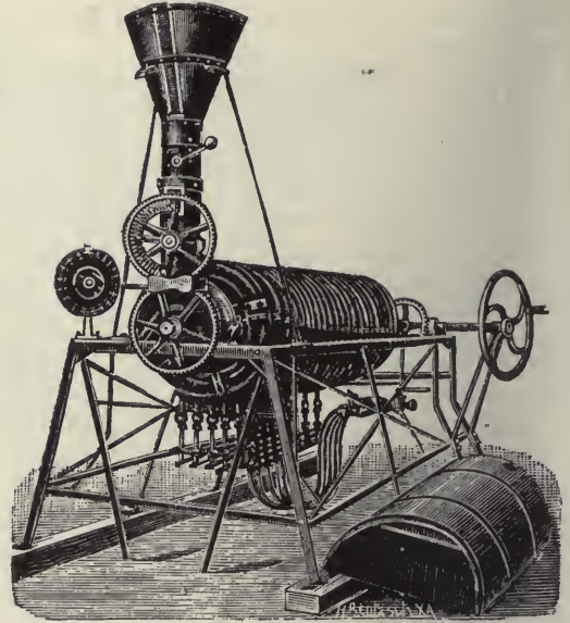
MAX THURMER'S QUICK GAS ROASTER
