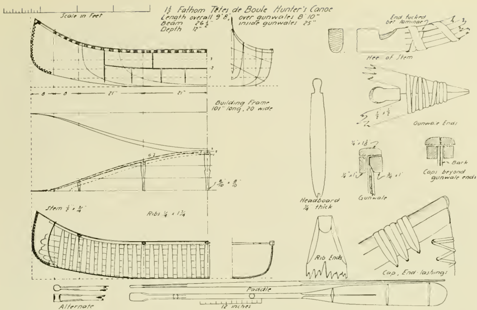
Figure 102 TÊTES DE BOULE HUNTING CANOE, 1 1/2-FATHOM, with typical construction details and a paddle.
