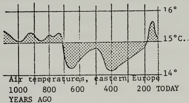
FIGURE 11 MEAN ANNUAL AIR TEMPERATURE CHANGES PAST 1000 YEARS
