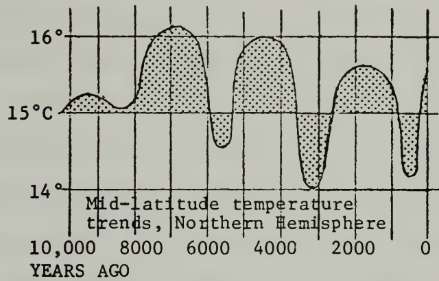
FIGURE 10 MEAN ANNUAL AIR TEMPERATURE CHANGES PAST 10,000 YEARS
