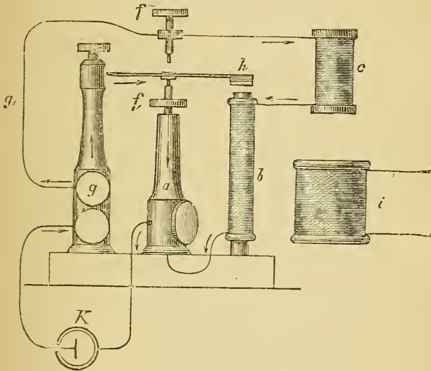
FIG. 74. HELMHOLTZ'S APPARATUS.
