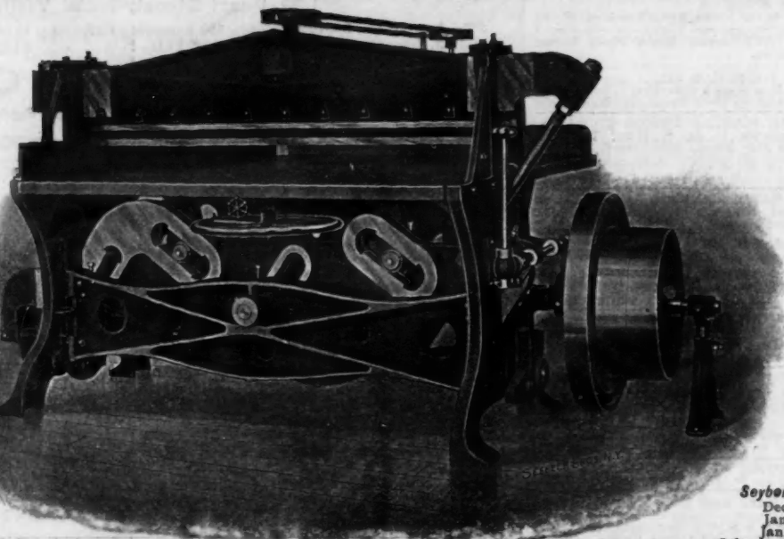
Holyoke Cutter—"Automatic Clamp," built in seven sizes, 24, 38, 44, 48, 54, 64 and 74 inches.
