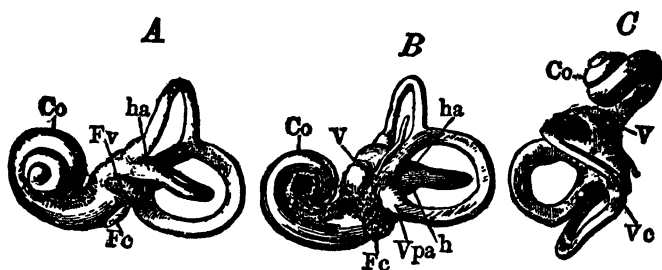
FIG. 19.—Casts of the bony labyrinth. A , left labyrinth seen from the outer side, B , right labyrinth from the inner side; C , left labyrinth from above; Co , cochlea; V , vestibule; Fc , round foramen; Fv , oval foramen; h , horizontal semicircular canal; ha , its ampulla; vpa , ampulla of posterior vertical semicircular canal; vc , conjoined portion of the two vertical canals.
