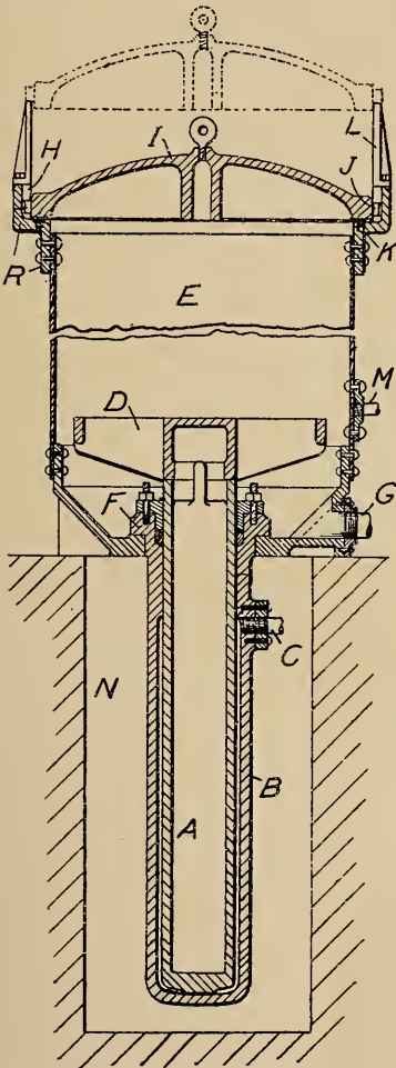
FIG. 173.—ADAMSON VULCANIZER PRESS
