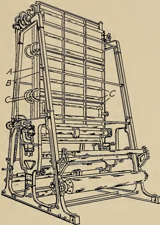
FIG. 207.—THE DECAUVILLE VERTICAL SPREADER.
