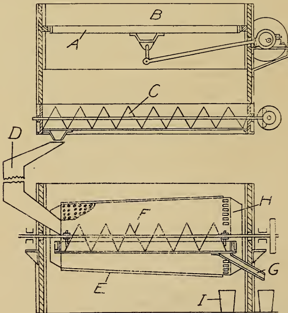
FIG. 302.—A GERMAN SEPARATOR.
