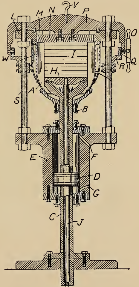
FIG. 174.—THE FILLINGHAM PRESS.
