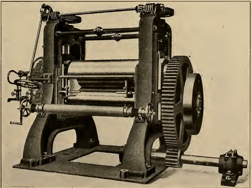
FIG. 85.—TWO-ROLL CALENDER.
