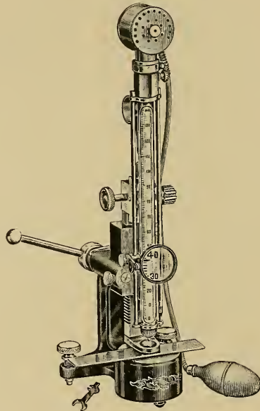
FIG. 418.—THE SHORE SCLEROSCOPE.
