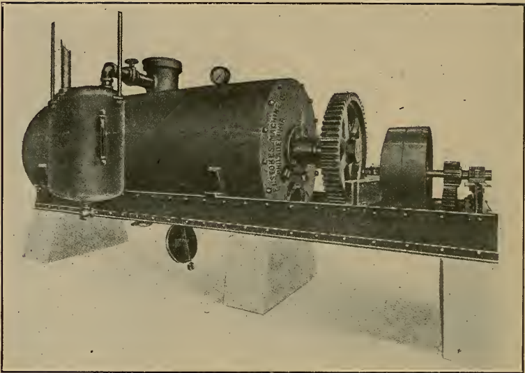
FIG. 333.—THE STOKES DRYER.
