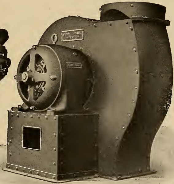
FIG. 27.—THE STURTEVANT BLOWER.
