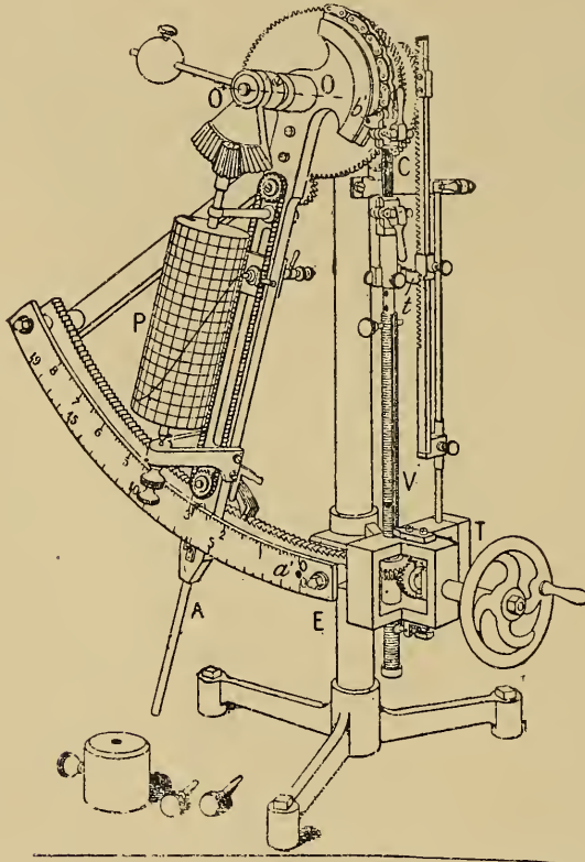
FIG. 422.—CHENEVEAU-HEIM RECORDING DYNAMOMETER.
