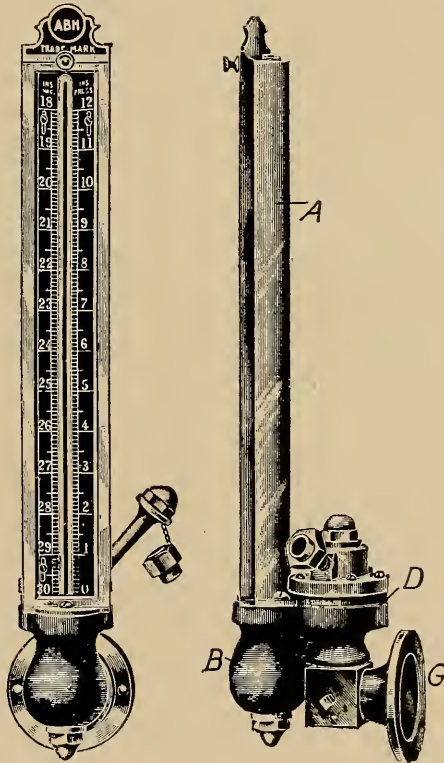
FIG. 350.—THE TAGLIABUE VACUUM GAGE.
