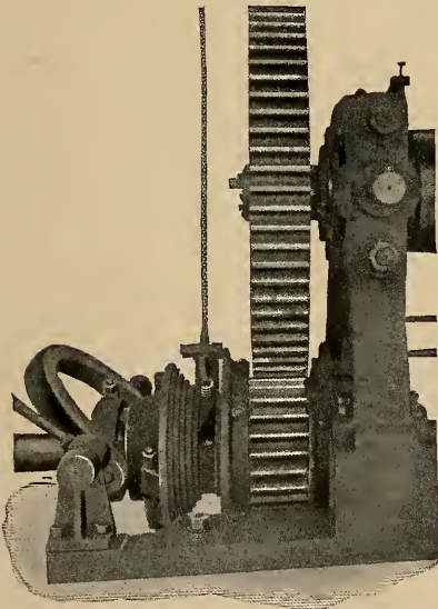
FIG. 118.—CLUTCH ENGAGED.
