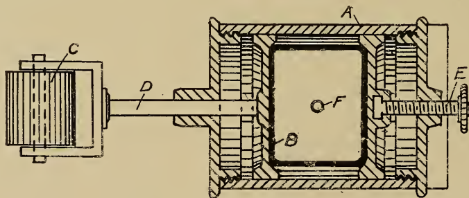
FIG. 98.—THE CLAREMONT CALENDER GAGE.
