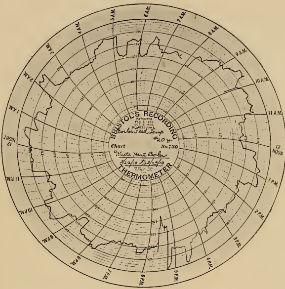
FIG. 363.—CHART MADE BY RECORDING THERMOMETER.
