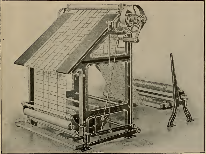
FIG. 81.—CLOTH INSPECTOR.
