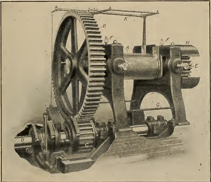
FIG. 4.—TWO-ROLL WASHER.
