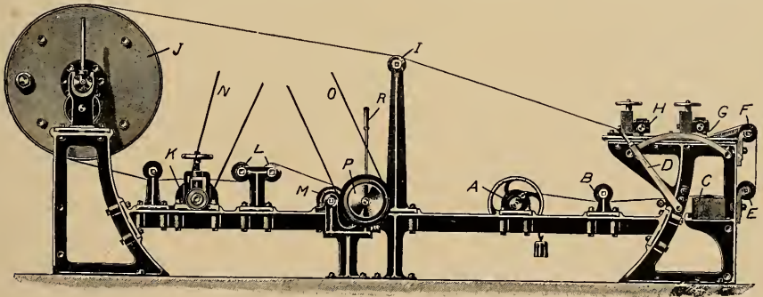
FIG. 227.—THE BRIDGE COLD CURE MACHINE.
