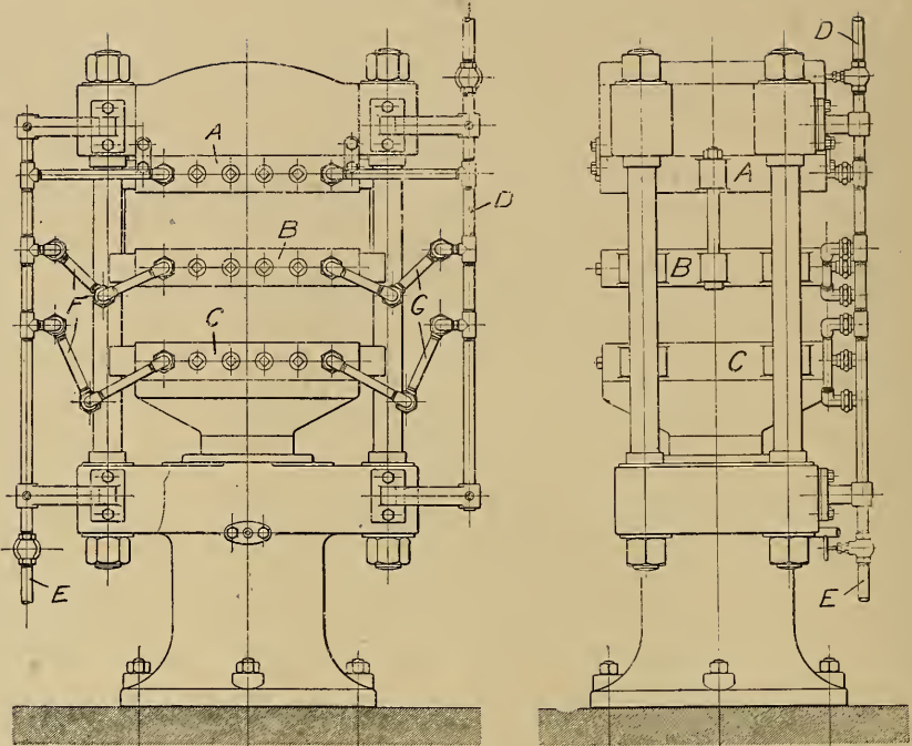
FIG. 168.—THREE-PLATEN PRESS.
