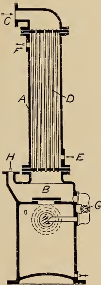
FIG. 30.—SURFACE CONDENSER.
