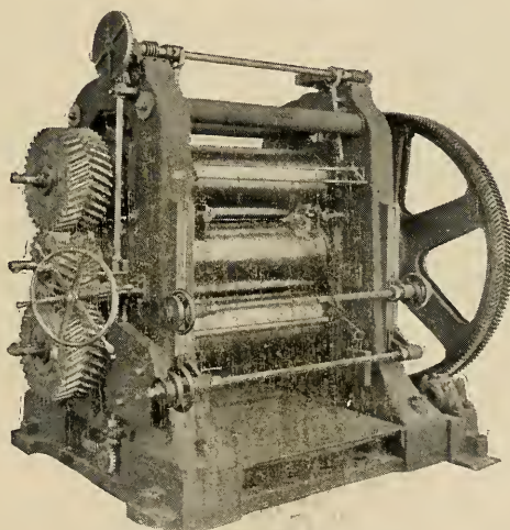
24" x 66" 3 ROLL CALENDER
