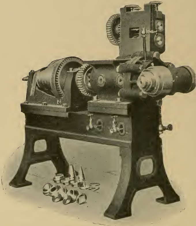
FIG. 187.—THE BRIDGE TUBING MACHINE FEED OPEN.
