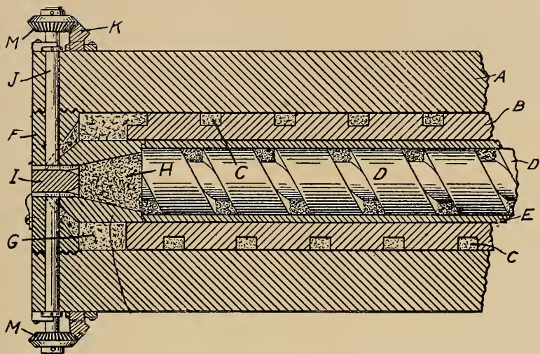
FIG. 188.—THE MAHONEY STRIPED TUBING MACHINE.
