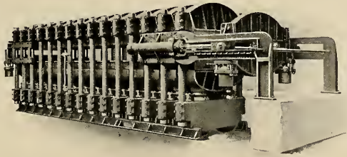
74" x 30' 6" Hydraulic Belt Press. Weight, 440,000 pounds.
