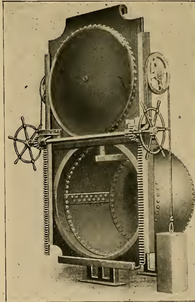
FIG. 160.—THE BRIDGE "AKRON-WILLIAMS" DOOR.
