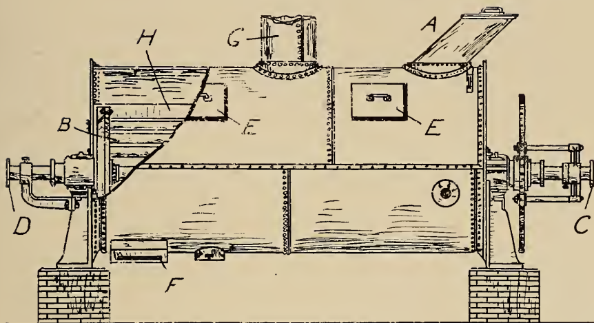
FIG. 41.—THE ROTARY DRYER.
