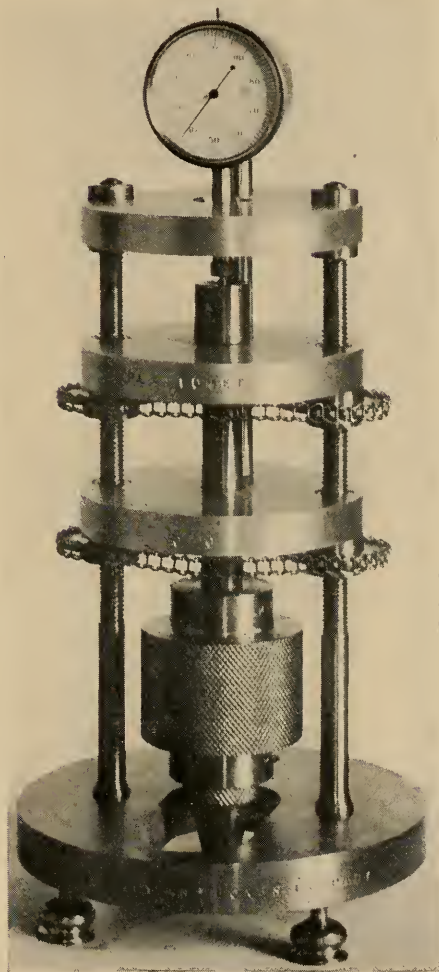
FIG. 417.—THE PLASTOMETER.
