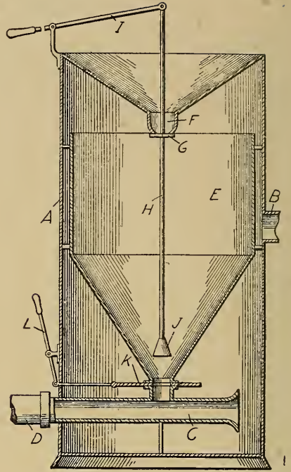
FIG. 140.—SAND-BLAST CLEANER.
