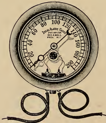
FIG. 355.—THE "IDEAL" GAGE.
