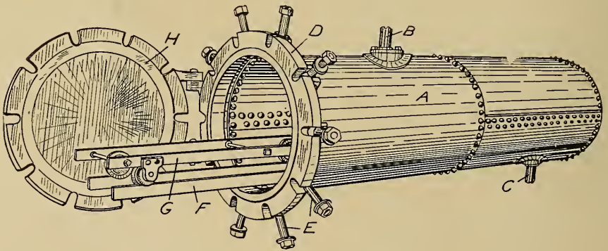
FIG. 141.—HORIZONTAL VULCANIZER.
