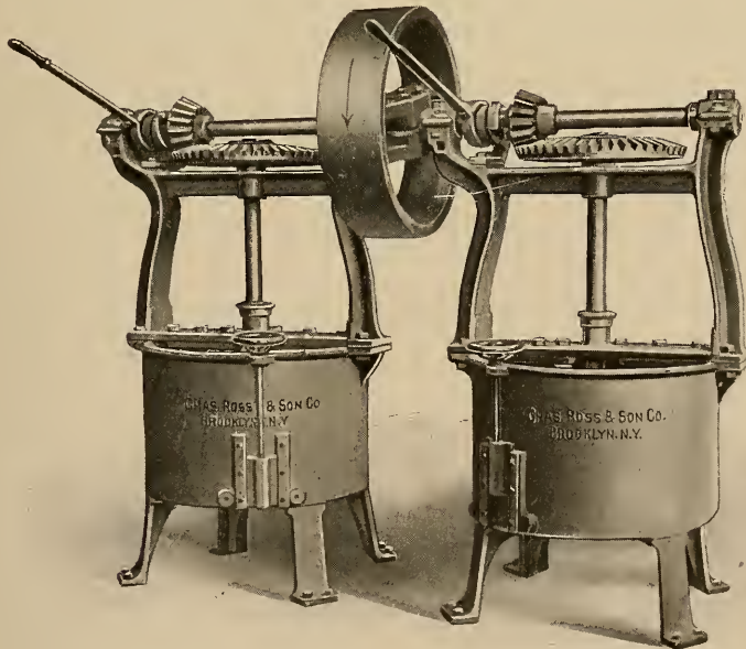
FIG. 246.—TWIN SOLUTION CHURNS.
