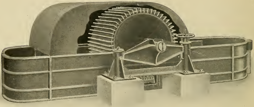
FIG. 6.—THE VAUGHN IRON TUB WASHER.
