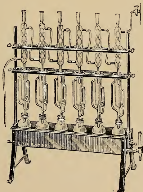
FIG. 380.—SOXHLET EXTRACTORS.
