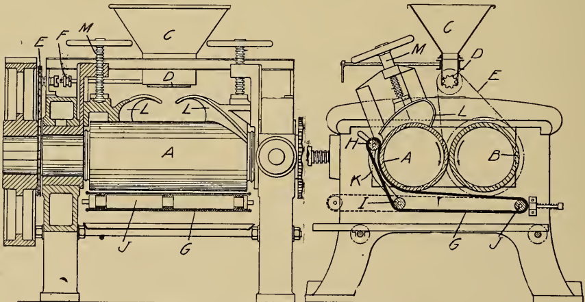
FIG. 60.—THE OLIER MIXER.
