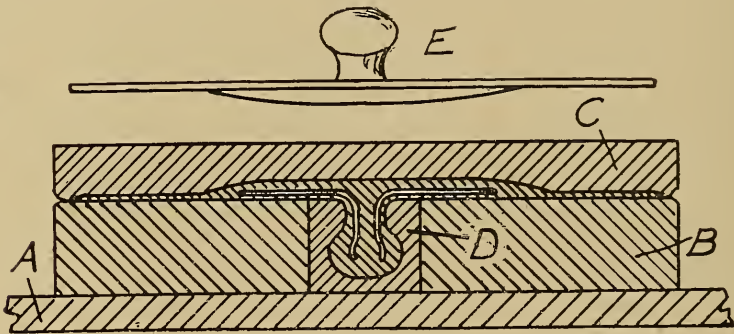
FIG. 135.—TYPE OF FIVE-PART MOLD.
