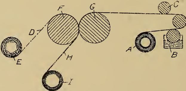
FIG. 220.—THE BIRNBAUM DOUBLER.
