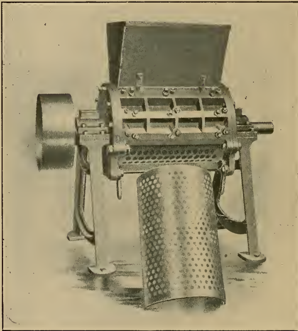
FIG. 294.—ROTARY CUTTER.
