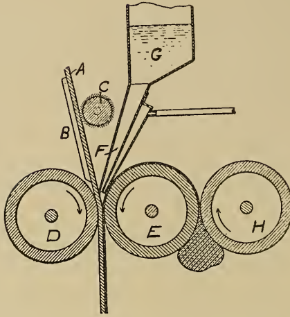
FIG. 92.—THE STEINHARTER LEATHER COATING CALENDER.
