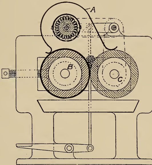
FIG. 53.—THE HAUBOLD MIXER WITH TRANSPARENT COVER.
