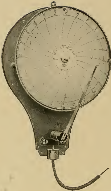
FIG. 361.—HELICAL RECORDER.
