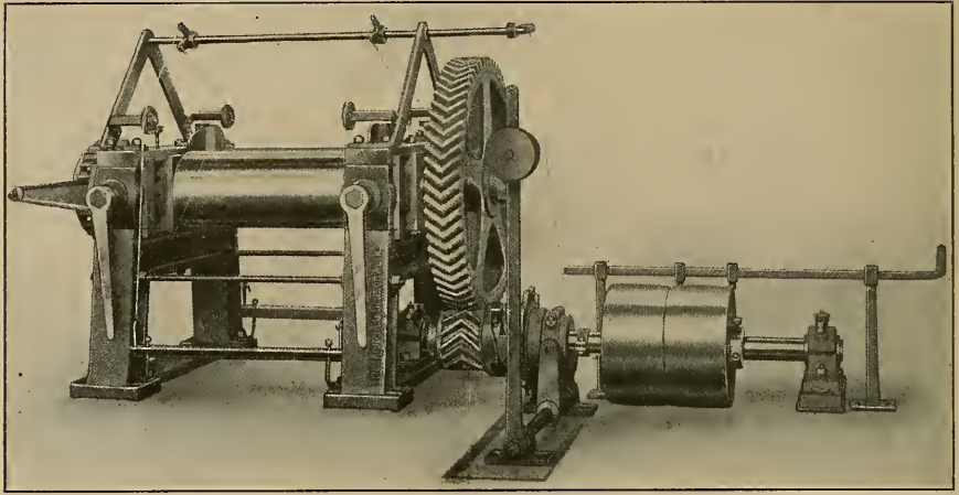
FIG. 125.—THE KRUPP SAFETY STOP.
