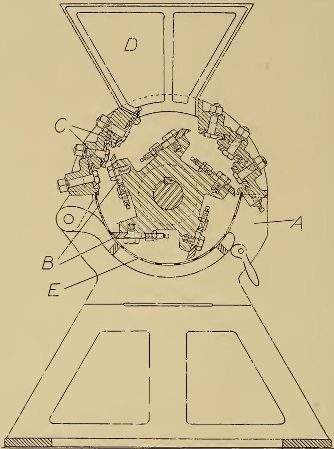
FIG. 260.—ROTARY CUTTER.
