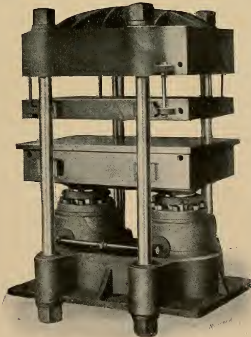
FIG. 169.—THE FARREL TWO-RAM PRESS.
