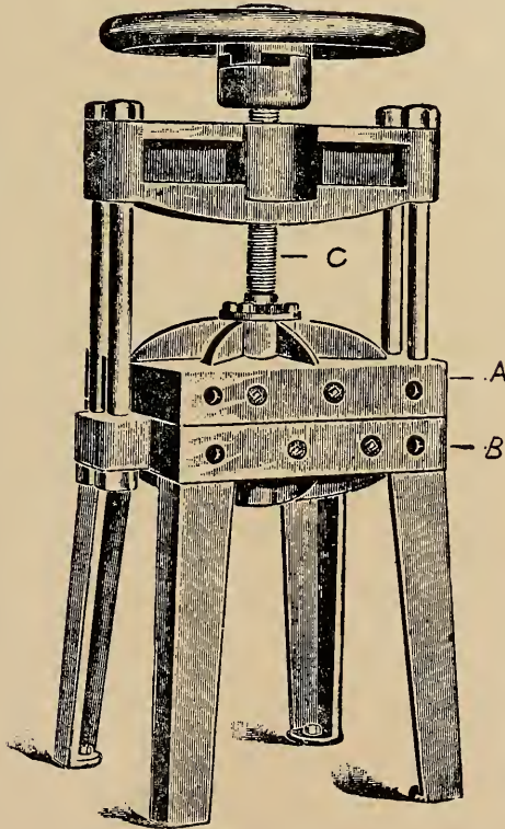
FIG. 163.—KNOCK PRESS.
