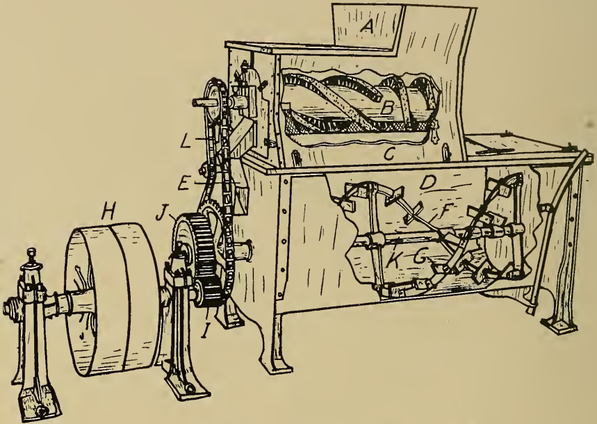
FIG. 33.—THE GAUNTT SIFTER.
