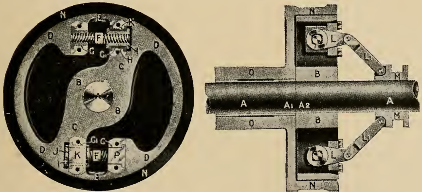
FIG. 105.—THE H. & B. FRICTION CLUTCH.
