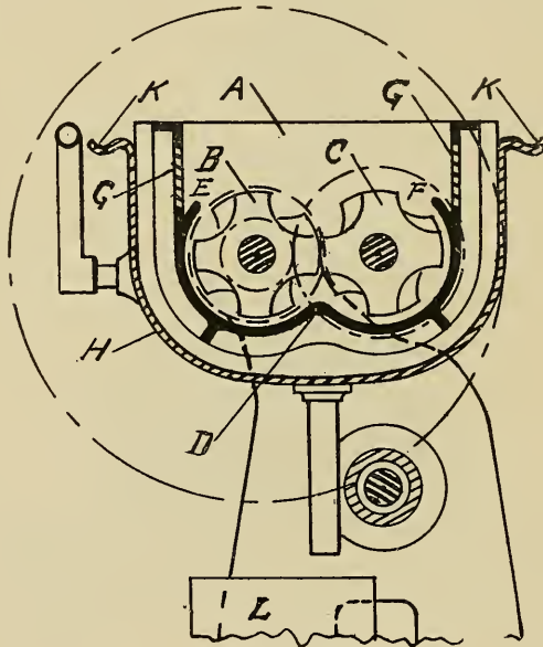
FIG. 13.—THE KEMPTER WASHER.
