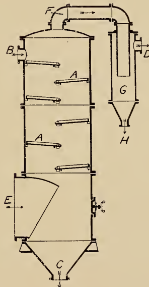
FIG. 31.—INJECTION CONDENSER.
