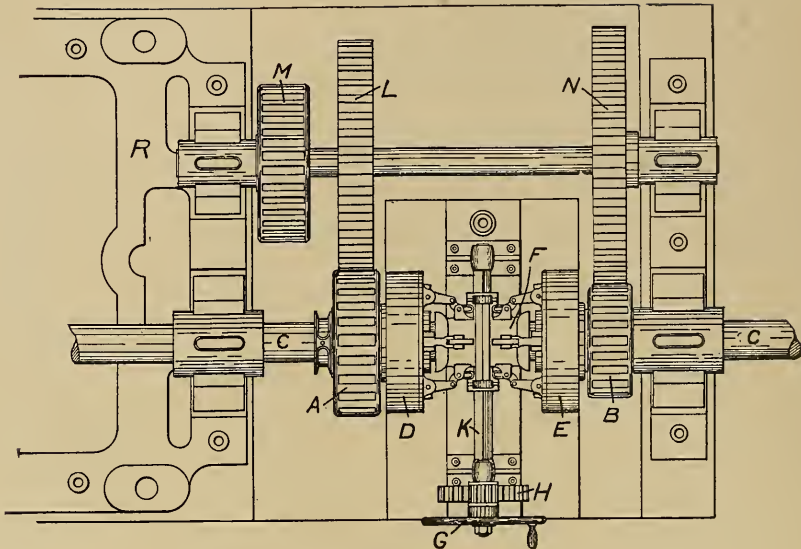
FIG. 112.—TWO-SPEED DRIVE.
