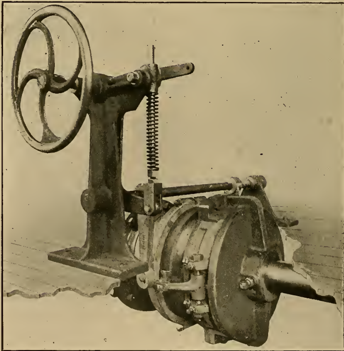
FIG. 106.—THE VAUGHN FRICTION CLUTCH.
