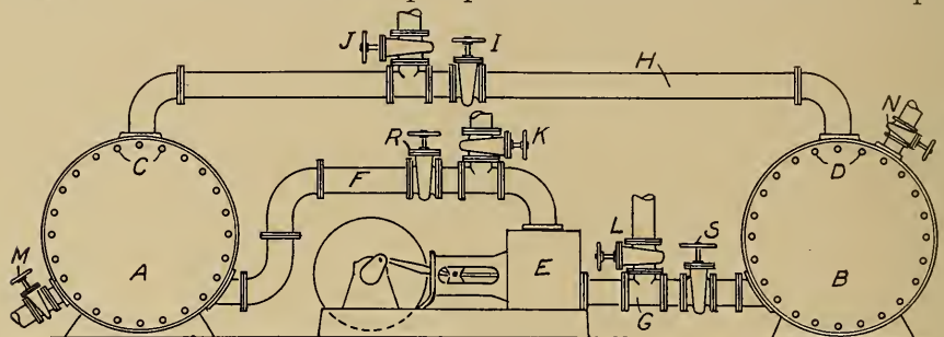
FIG. 148.—THE WITTENBERG VULCANIZER.
