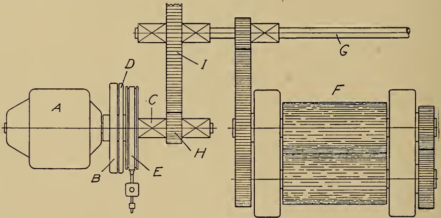
FIG. 110.—CLUTCH AND BRAKE INSTALLATION.
