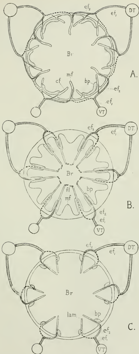
Fig. 78. Diagrammatic t.s. through branchial basket of Anisopterid larvae, to show types of gill-system. A. Undulate Simplex. B. Foliate Duplex. C. Lamellate Duplex. bp basal pad; Br branchial basket; cf cross-fold; DT dorsal trunk; ef 1 primary, ef 2 secondary efferent; fl foliae; lam lamellae; mf main-fold; VT visceral trunk. In c, only one lamella is shown cut in each hemibranch, although six or more are really cut (see fig. 83 B). The dotted tracheae lie outside the true level of the section. Original.
