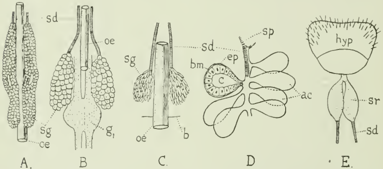
Fig. 45. Salivary glands. A. Libellula depressa Linn. B. Platycnemis pennipes Pallas. C. Agrion puella Linn. D. Lestes viridis Vand. E. Calopteryx virgo Linn., reservoirs. ac acini; b posterior border of prothorax; bm basement membrane; c lumen of acinus; ep epithelium of acinus; g 1 prothoracic nerve-ganglion; hyp hypopharynx; oe oesophagus; sd salivary duct; sg salivary gland; sp spiral ridge of intima of duct; sr salivary reservoir. In D the top left-hand acinus is shewn in section, and only a small portion of the whole gland is shewn, much enlarged. After Bordas.
