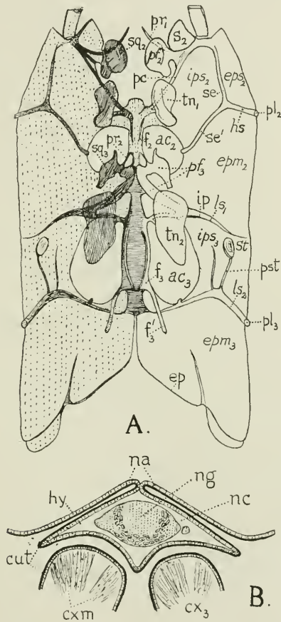
Fig. 8 A. Internal ventral view of skeleton of a Dragonfly's thorax, to shew endoskeleton. Adapted from Berlèse. B. T.S. through metathoracic neural canal in Isosticta simplex Martin ( \times 15 ). Original. ac acetabulum; cut cuticle; cx 3 metacoxa; cxm coxal muscles; hy hypoderm; na sternal apodemes; nc neural canal; ng metathoracic ganglion; st metastigma. For references to parts of endoskeleton, see text; to exoskeleton, legend of fig. 1.
