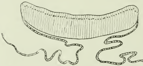
Fig. 50. Lateral sagittal section through epithelium of one of the pads of the pre-rectal ampulla, from larva of Libellula ( \times 50 ). After Sadones.
