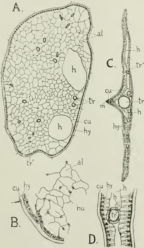
Fig. 86. Histology of the caudal gill. A. T.S. through basal third of saccus of Diphlebia lestoules Selys ( \times 47 ). B. Small portion of same ( \times 200 ). C. T.S. through basal third of lateral lamellar gill of Synlestes weyersi Selys ( \times 47 ). D. Small portion of same ( \times 200 ). al alveoli; b blood-plasma; cu cuticle; h haemocoel; hy hypoderm; nu nucleus of alveolus; tr main longitudinal trachea; tr' branch trachea. Original.
