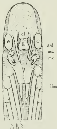
Fig. 112. Anterior half of egg of Anax papuensis Burm., just before hatching, ventral view ( \times 60 ). ant antenna; cl elypeus. e compound eye; lbm labium; lbr labrum; md mandible; mx first maxilla; p 1 -p 3 legs. Original.
