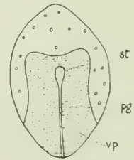
Fig 110. Ventral plate ( vp ) and primitive groove ( pg ) in Libellula . st stomodaeum. After Heymons.
