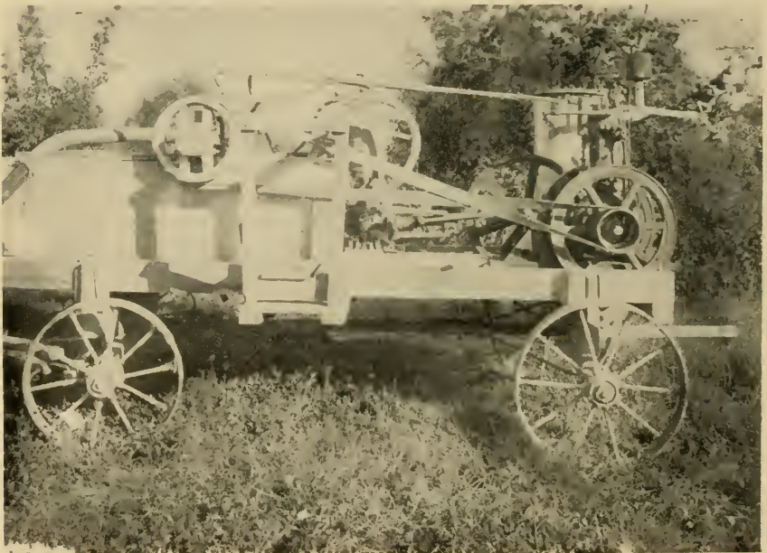
2. PRIMITIVE TYPE OF GASOLINE POWER SPRAYER, USED IN THE EARLY TWENTIETH CENTURY FOR CODLING MOTH CONTROL.
