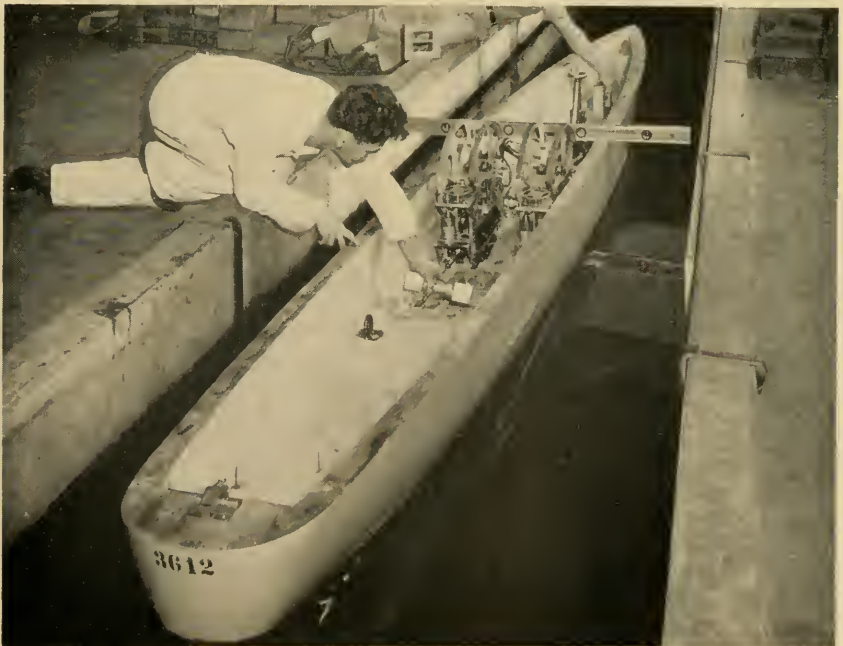
2. DAVID W. TAYLOR MODEL BASIN
