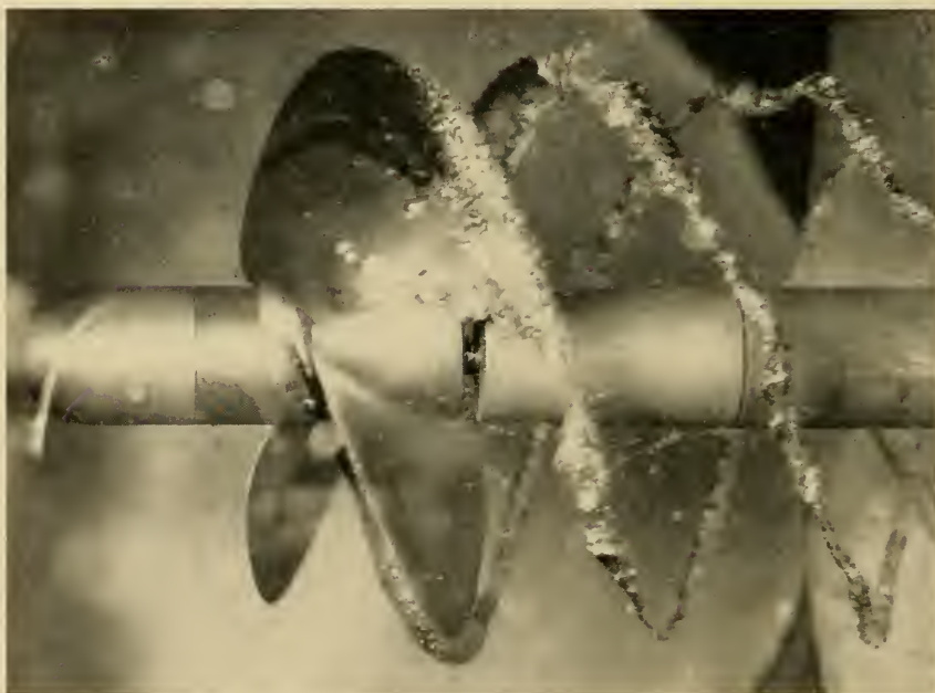
2. CAVITATING MODEL PROPELLER UNDER TEST IN 12-INCH WATER TUNNEL.
