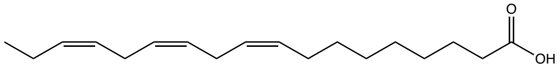
\alpha -linolenic acid
