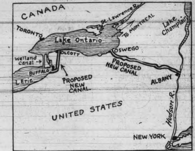
PROPOSED CANAL FROM LAKE ERIE TO NEW YORK. A bill to give private interests the right to construct such a waterway is now before the American Congress. The plan is to cut a canal through from Lake Erie, south of Buffalo, to Lake Ontario, and another from Oswego to Albany. A diversion of 30,000 cubic feet per second would be required for the canal, from Lake Erie. The proposal is not regarded as satisfactory to this country.
