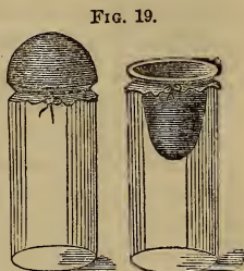
FIG. 19. Passage of gases through membranes.
