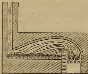
Reverberatory Furnace.
