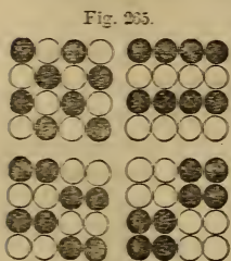
Illustration of Isomerism.
