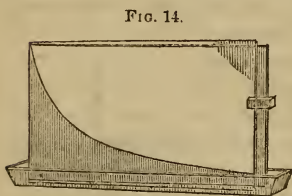
Rise of liquid between plates.
