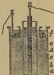
Daniell's cell.
