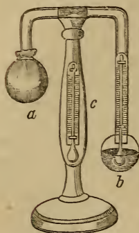
Daniell's Hygrometer.
