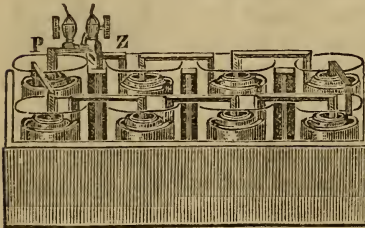
Grove's battery.
