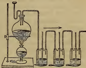
Woulfe's Bottles.
