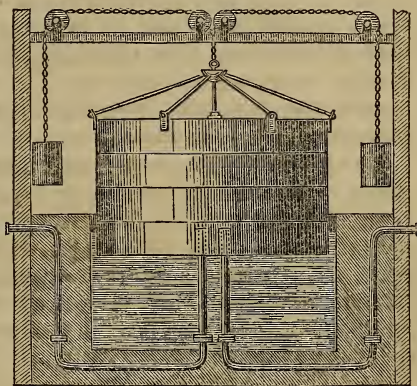
The Gasometer.
