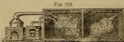
Manufacturing Sulphuric Ac.d.
