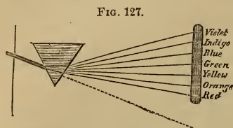
Decomposition of Light.
