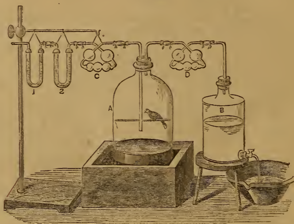
Measuring the Carbonic Acid exhaled by a Bird.
