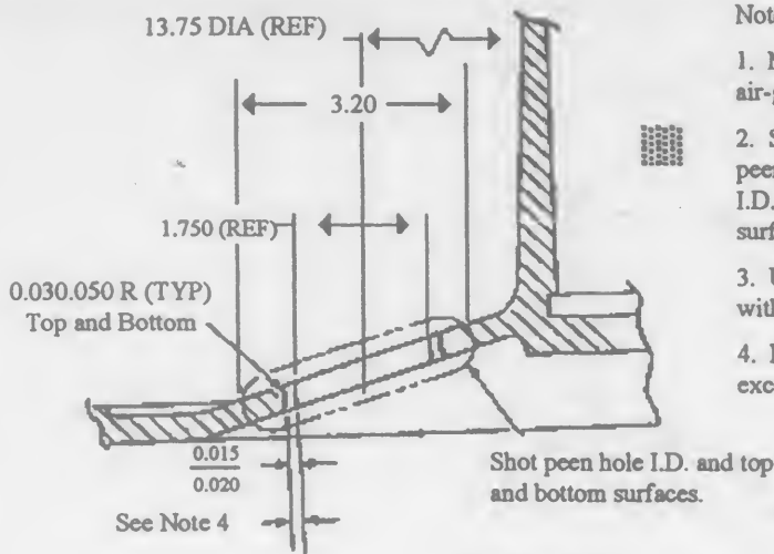
Section B-B (Typical Nine Places)
