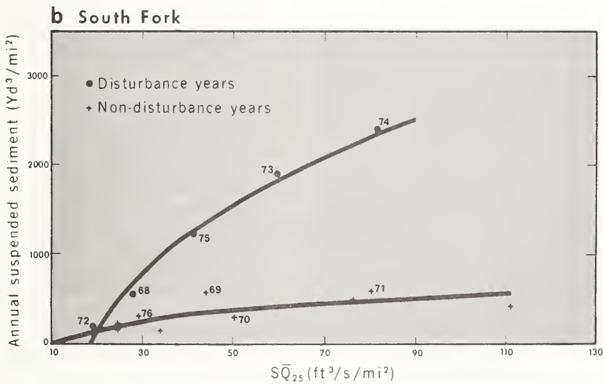
Annual sediment discharge of the forks as related to stream power as indexed by Q_{25} (the mean discharge for the top 25 percent of the flow volume).
