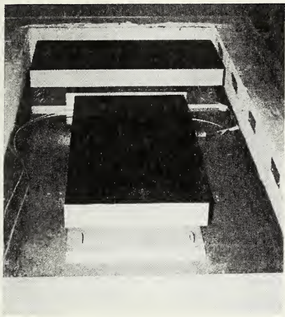
Figure 12. Two AMTI force plates on their air bearing carriers, resting on a hardened epoxy surface. Floor panels (not shown) are positioned around the force plates for actual gait testing. Photograph is courtesy of Advanced Mechanical Technology, Inc. (AMTI) and is used with permission.
