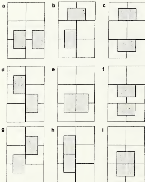
Figure 10. Floor panel cutout scheme, which allows two force plates to be arranged within a 4-ft wide by 6-ft long area, in 9 configurations (a through i). Four of the 2-ft square floor panels must have one corner removed to accommodate the force plates (shown in gray). One configuration (h) requires two corner notched floor panels and one additional narrow floor panel strip along the left side.
