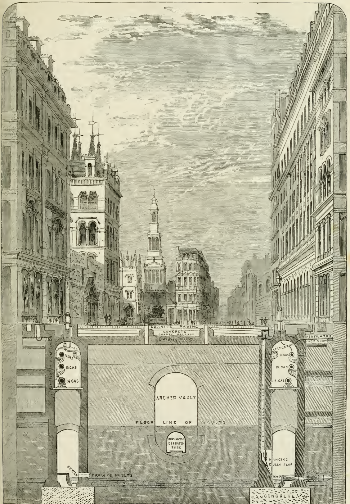
SECTION OF THE HOLBORN VIADUCT, SHOWING THE SUBWAYS. (Taken by permission from Mr. Haywood's Report.)
