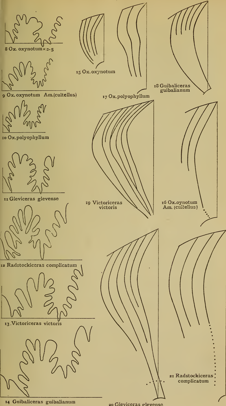
Figs. 8-21.—Suture-lines (skeleton) and radial lines of Oxynotoids.
