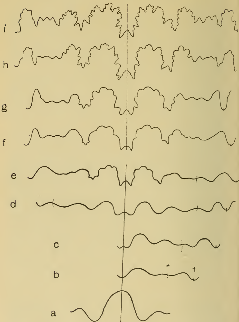
Fig. 9.— Development of the suture-line of Dactyloceras commune (figured in Pl. II, fig. 2).
