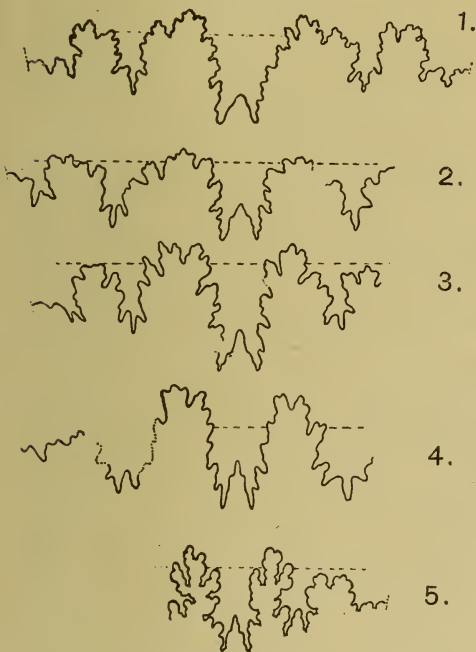
Fig. 8.— Suture-line of Dactylioceras and Cœloceras.
