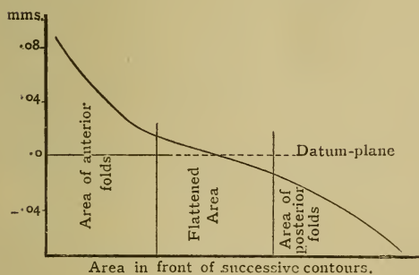
Fig. 7.—Graph illustrating the average profile of the second septum of Dactylioceras shown in Pl. III, fig. 4.
