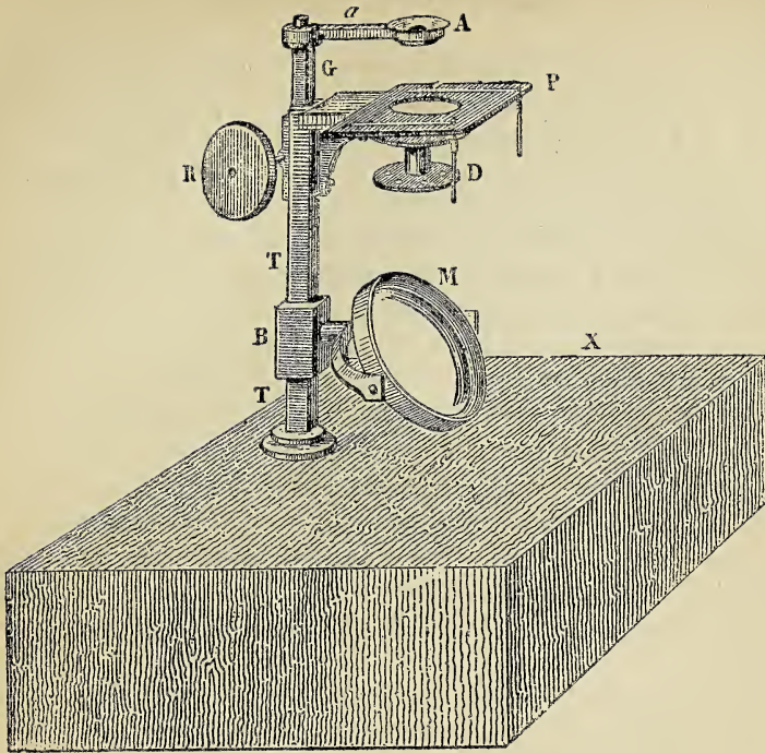
Fig. 15.—SIMPLE MICROSCOPE.
