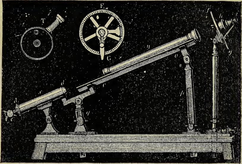
Fig. 35.—BIOT'S POLARISCOPE.
