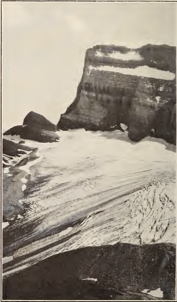
FIG. 7.—GOULD MOUNTAIN AND GRINNELL GLACIER.
