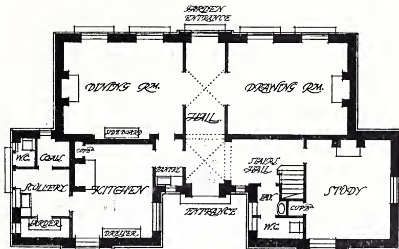
PLAN OF HOUSE AT HARPENDEN
