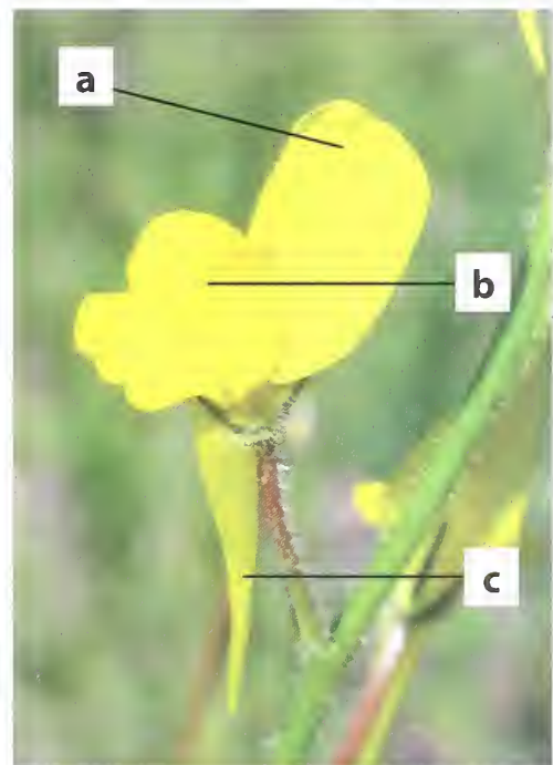
Figure 4. Yellow toadflax ( Linaria vulgaris ) flower. (a) Upper lip, (b) lower lip, (c) spur.
