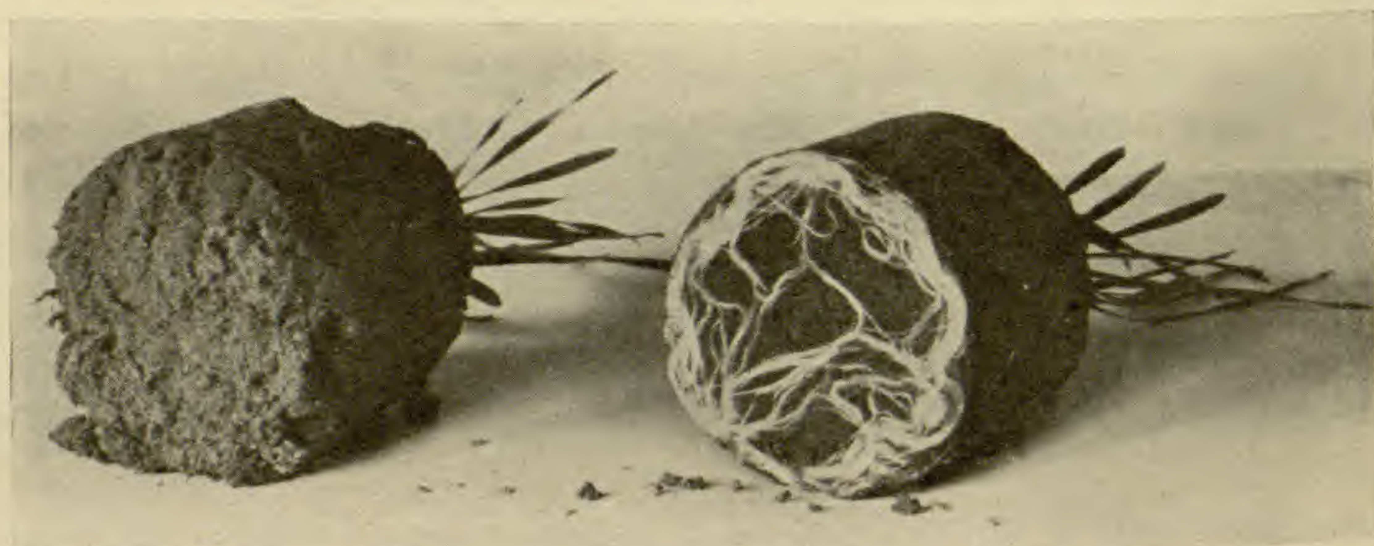
FIG. 2.—Root distribution in paraffined wire pot and in ordinary pot; on the left is shown the contents of a paraffined wire pot, and on the right those of an ordinary pot.
