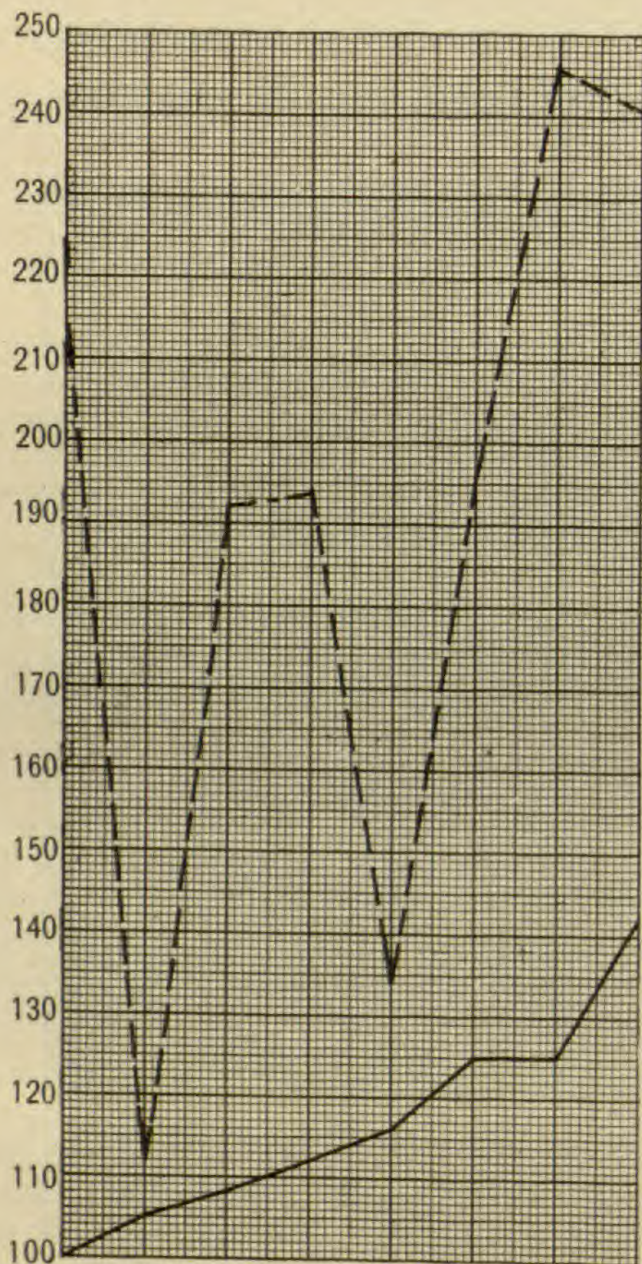
FIG. 9.—Correlative growth and transpiration in soil extracts to which \text{CaCO}_3 was added.
