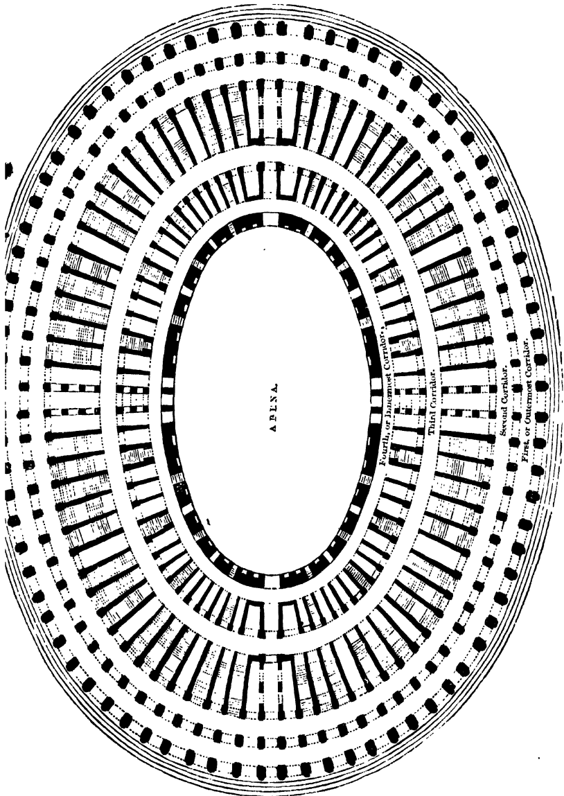
GROUND-PLAN OF THE FLAVIAN AMPHITHEATRE.
