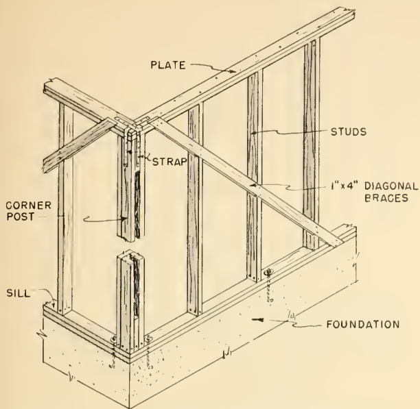
FIGURE 28.—Diagonal bracing and steel strapping used to strengthen end walls.
