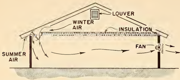
FIGURE 21.—Fan on sidewall drawing air from attic in winter. In summer, attic space is closed and outdoor air is brought into house through slot opening at eave.
