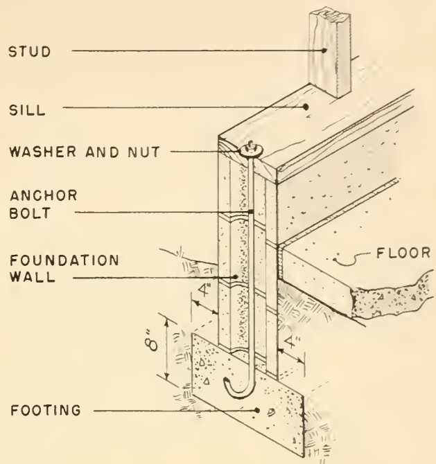
FIGURE 25.—Detail of foundation and footing. Note that anchor bolt extends into footing.
