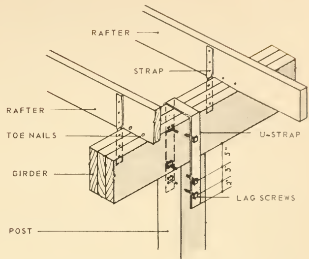
FIGURE 30.—U-strap, 2 \frac{1}{4} -by \frac{3}{16} -inch, used to tie girder to post.
