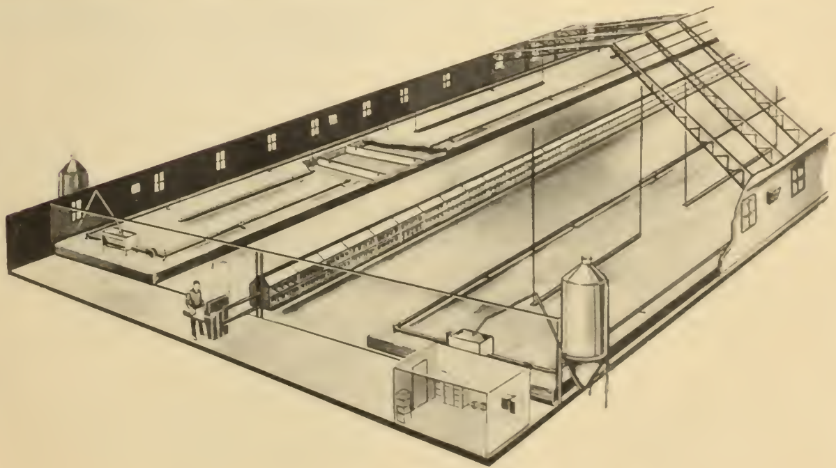
FIGURE 3.—Automated laying house with mechanical feeders and waterers above a raised platform and with partial wood-slat floors.
