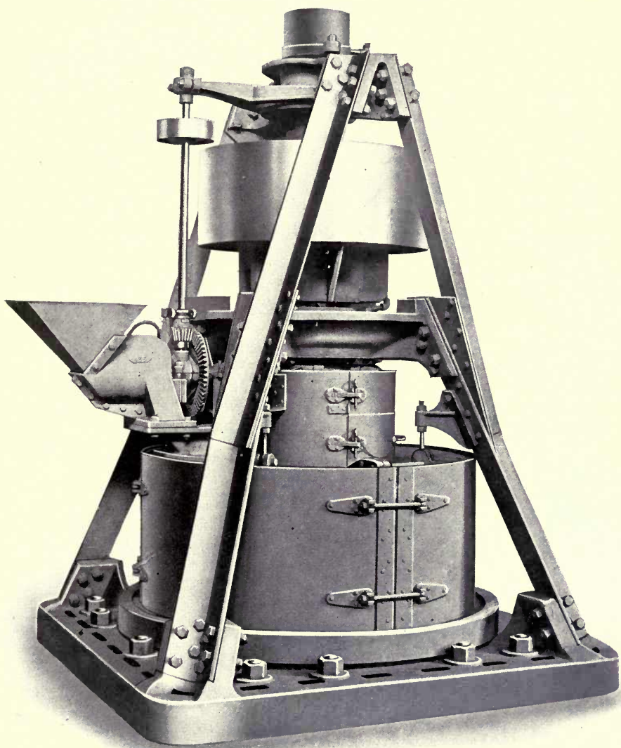
Griffin mill.
