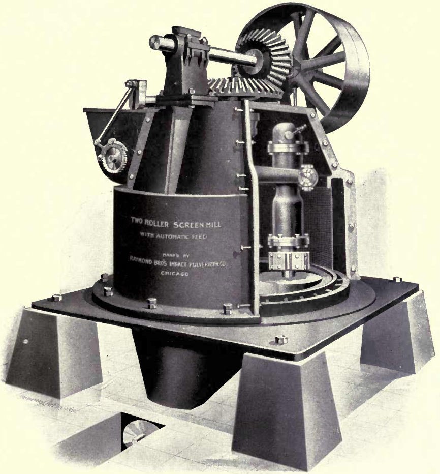
Raymond mill.
