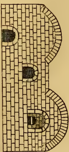
End view of the Platting Ovens.
