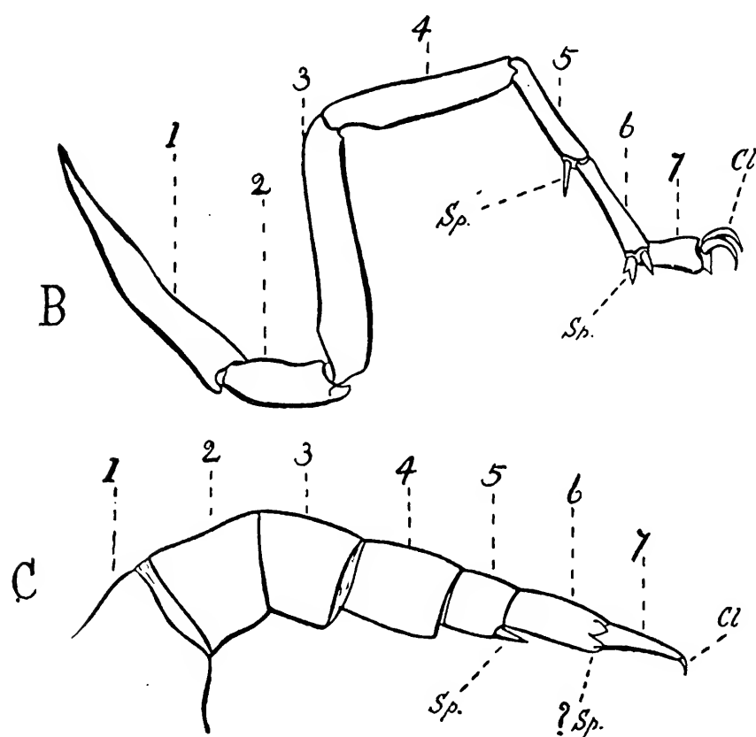
Figure 28 B, fourth leg of a recent scorpion ( Butkus australis ); C, third leg of Siluric scorpion ( Palaeophonus nunciatus ). (From Pocock)
