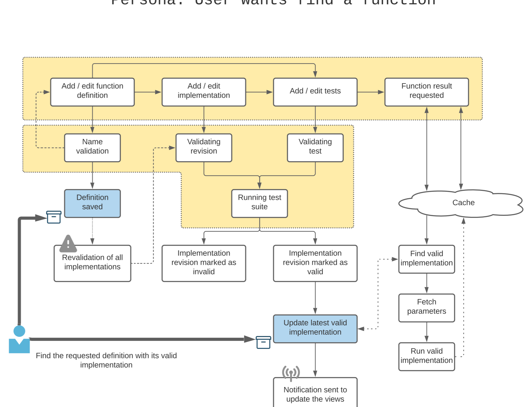
Persona: User wants find a function
