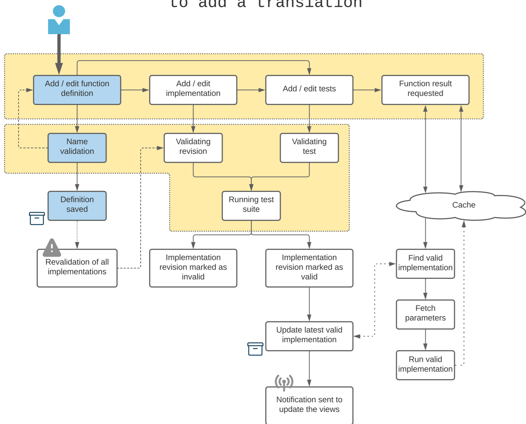
Persona: User wants to edit the definition to add a translation
