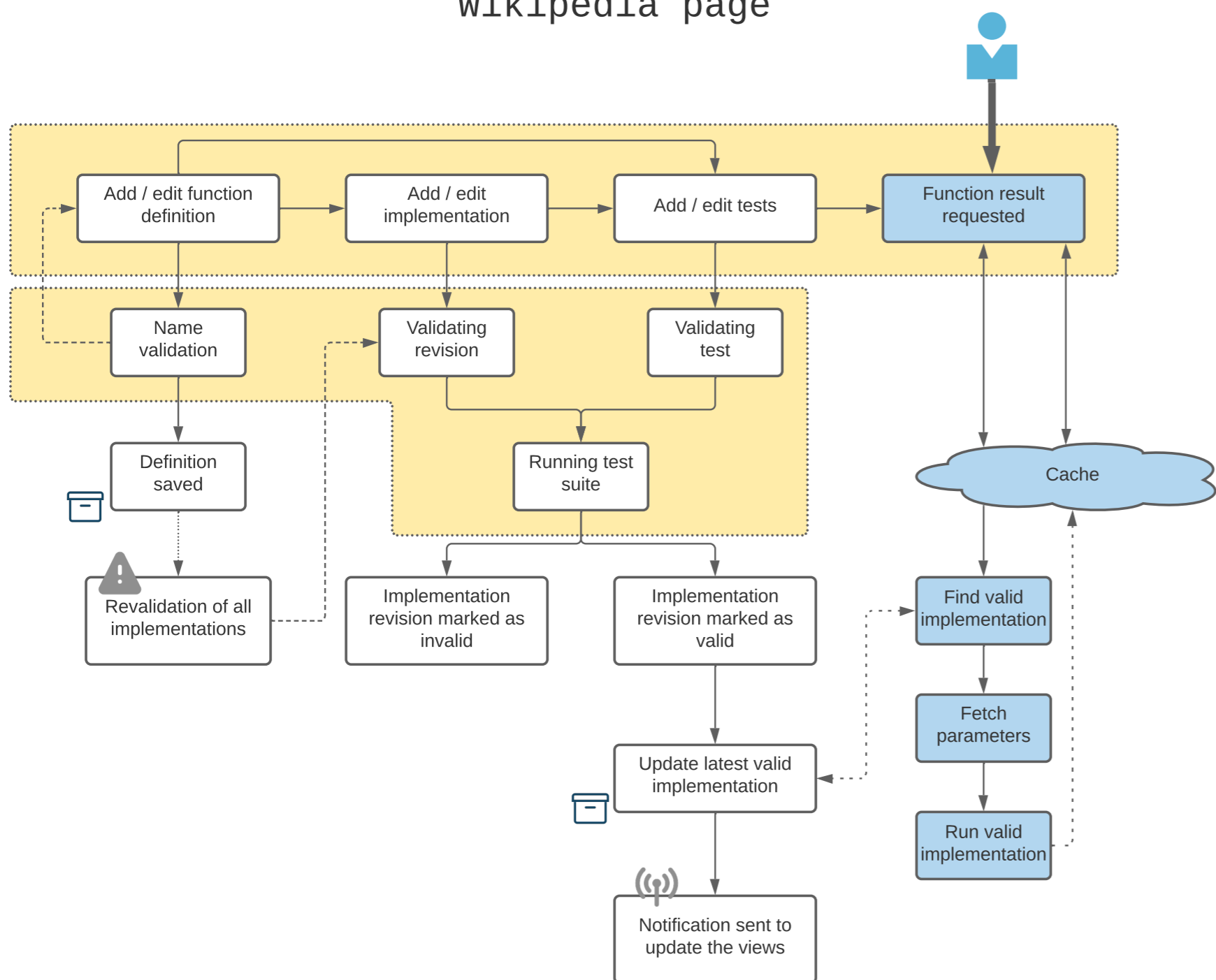
Persona: User wants to run a function from a Wikipedia page
