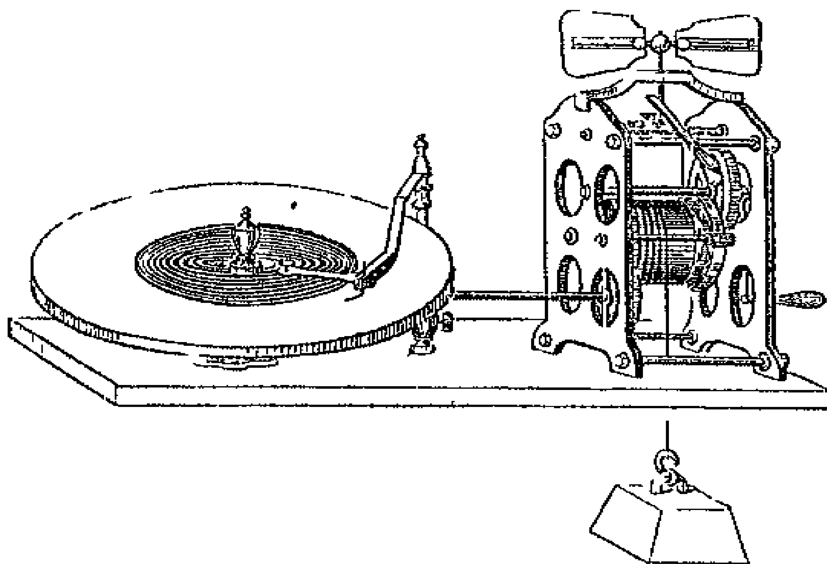
Fig. 87.—BAIN'S ELECTRO-CHEMICAL TELEGRAPH
