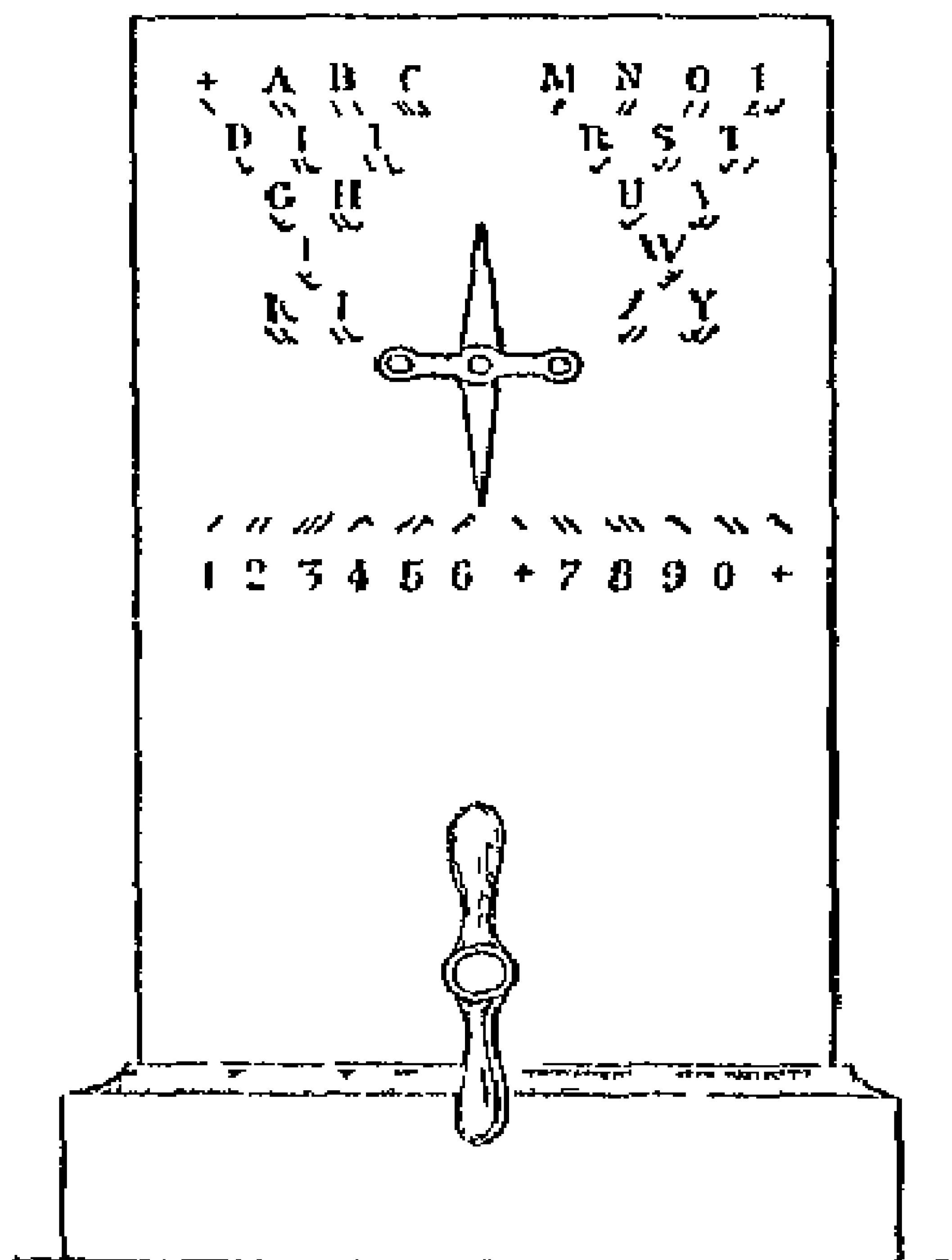
Fig. 68.—THE SINGLE NEEDLE TELEGRAPH.
