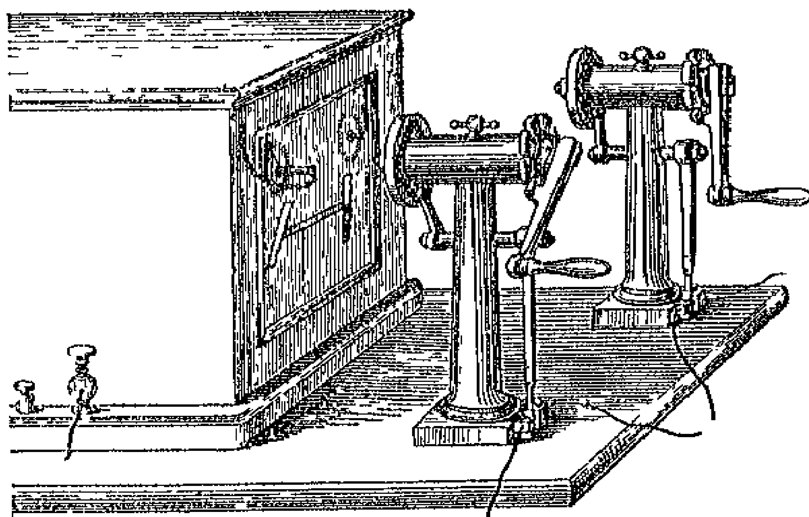
Fig. 73.—FRENCH STATIC TELEGRAPH
