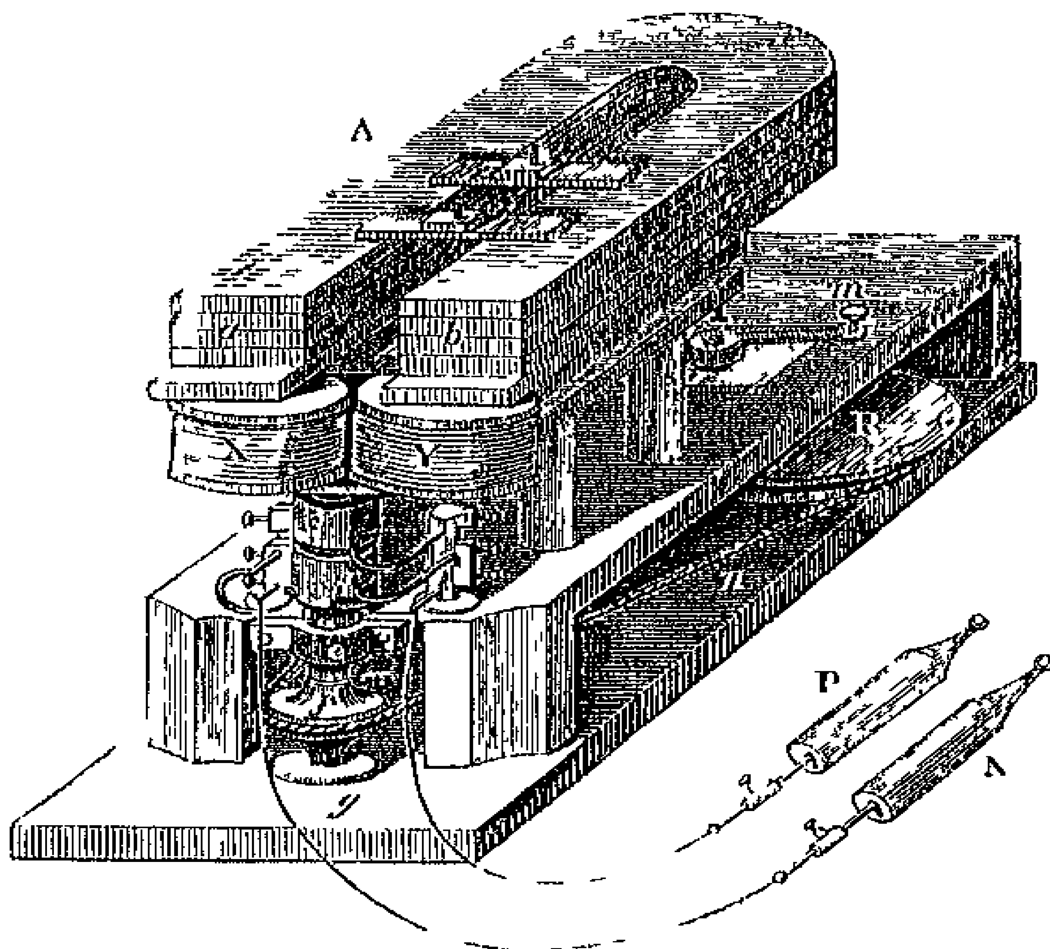
Fig. 61 —MAGNETO ELECTRIC MACHINE
